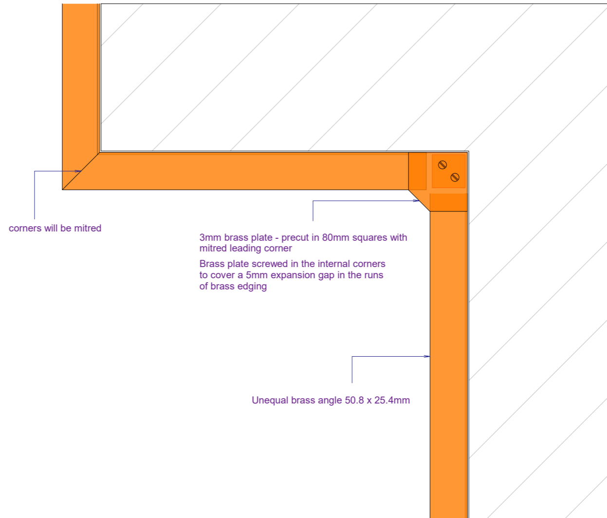
FLOOR PLAN DETAIL - SHOWING INTERNAL CORNER DETAIL
