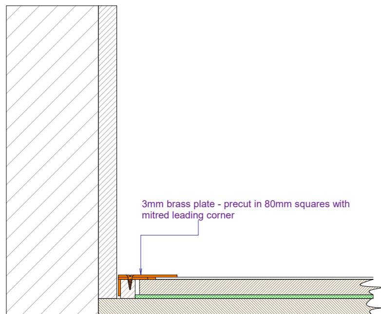
FLOORING SECTION - SHOWING INTERNAL CORNER DETAIL
