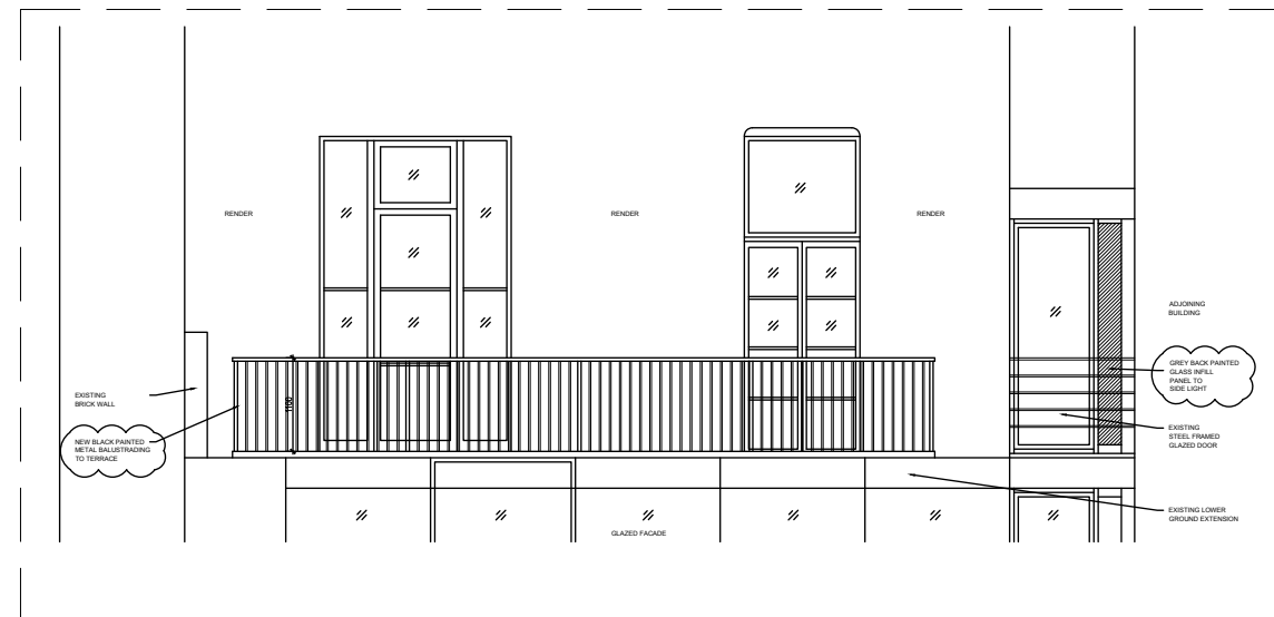
PROPOSED REAR ELEVATION ( GROUND FLOOR )
