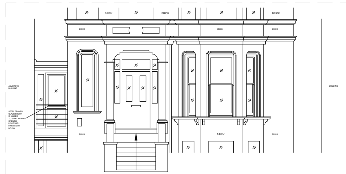
PROPOSED FRONT ELEVATION ( GROUND FLOOR )
