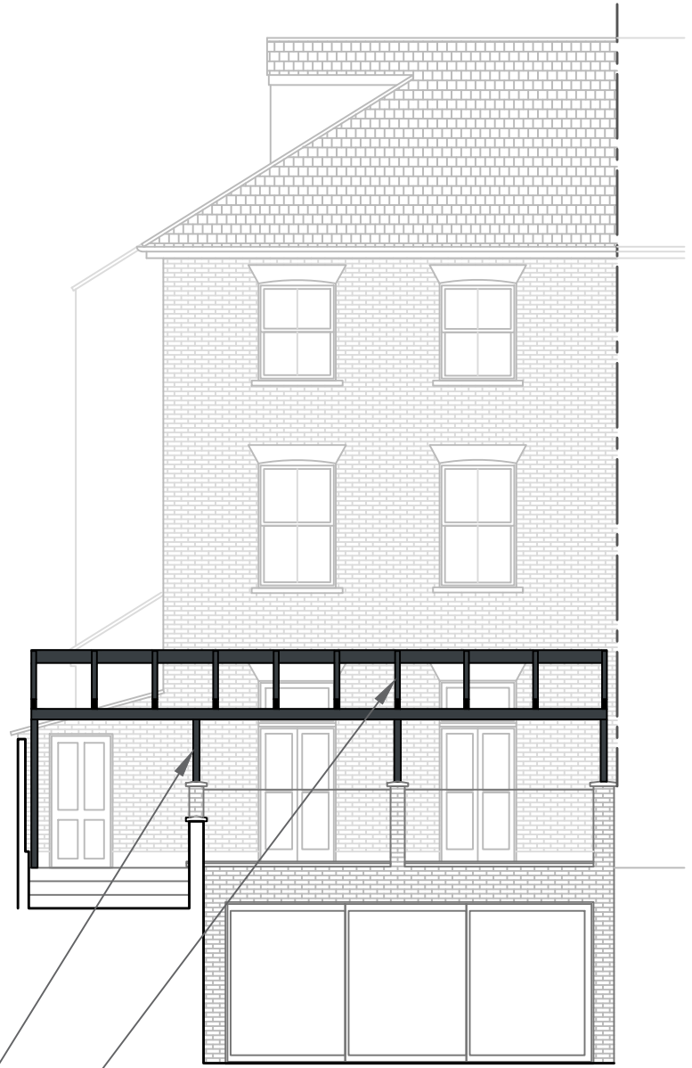
Rear Elevation
