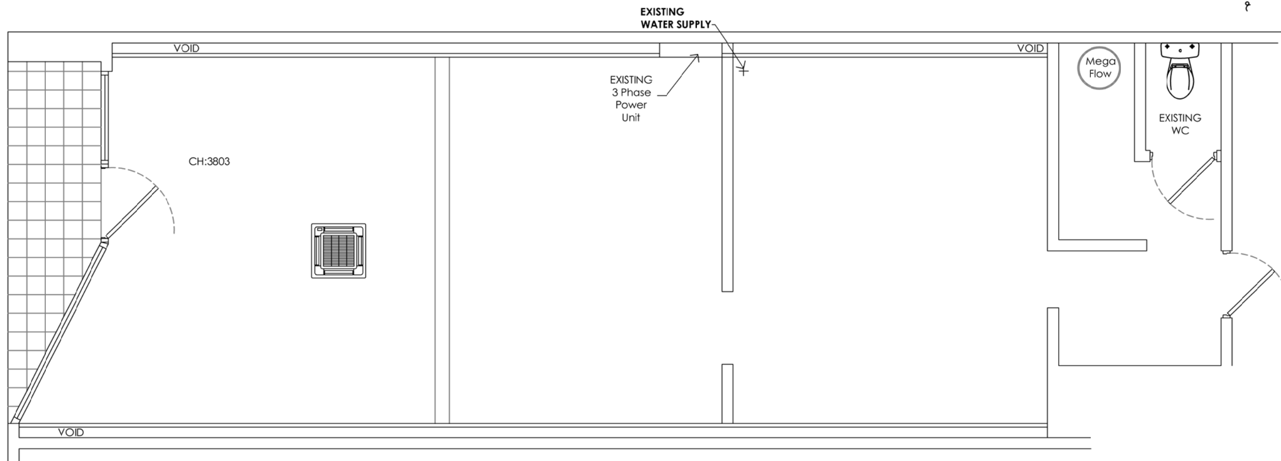
EXISTING FLOOR LAYOUT - SCALE 1:50
