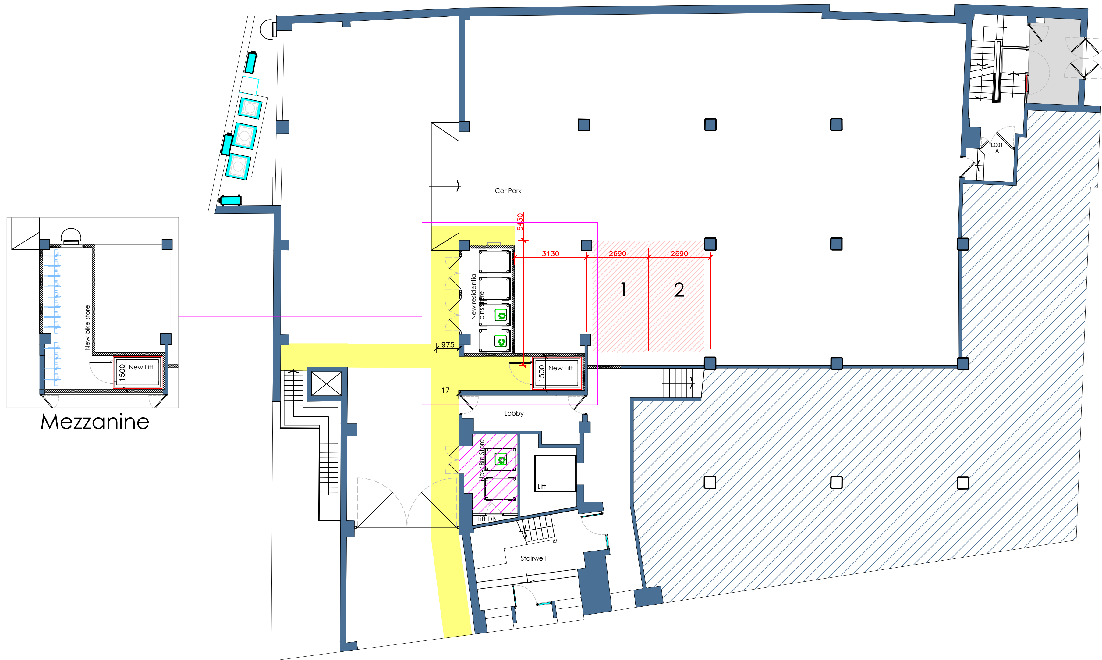
GROUND FLOOR PROPOSED LAYOUT
