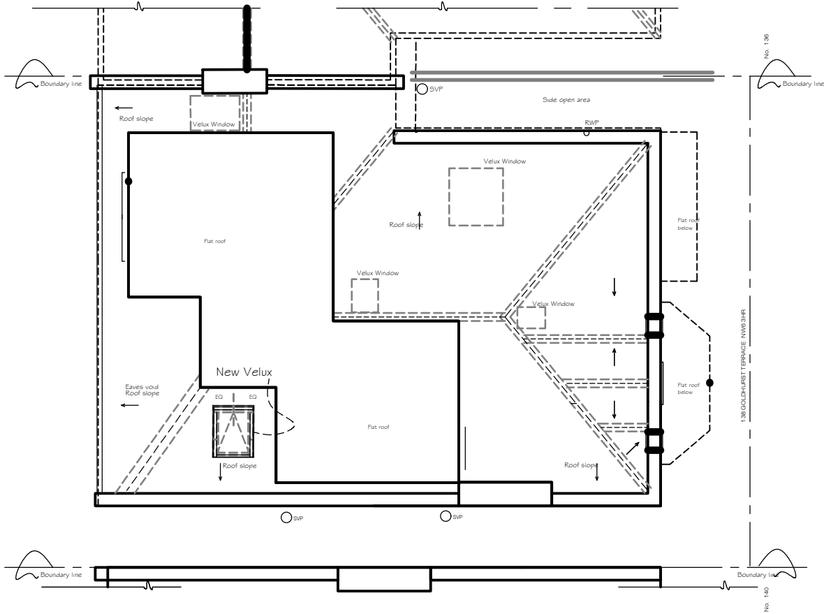
PROPOSED ROOF PLAN GENERAL ARRANGMENT
