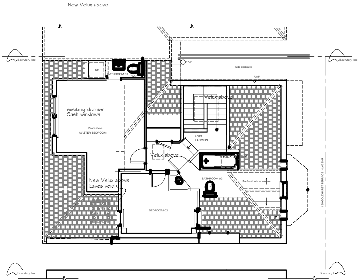
PROPOSED LOFT PLAN GENERAL ARRANGMENT
