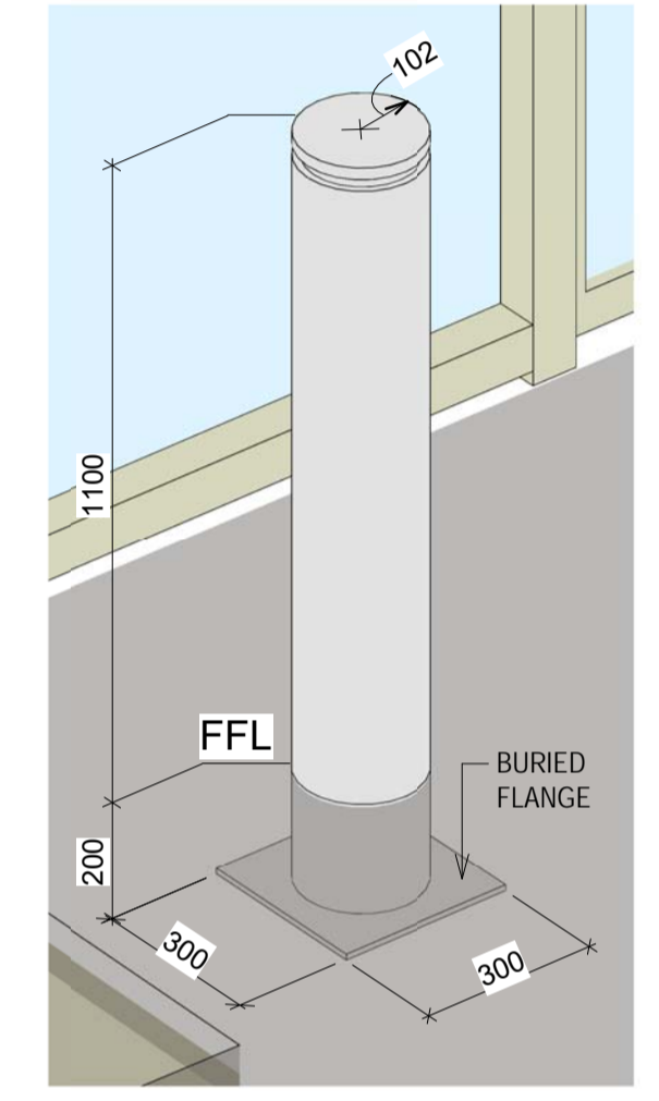
4 MARSHALLS BOLLARD GE-BL-00011
