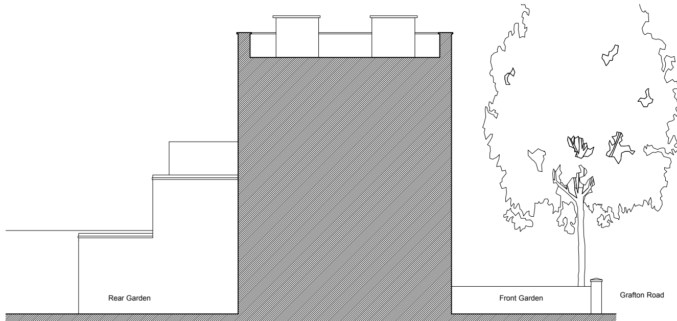
SIDE ELEVATION FROM 29 GRAFTON ROAD
