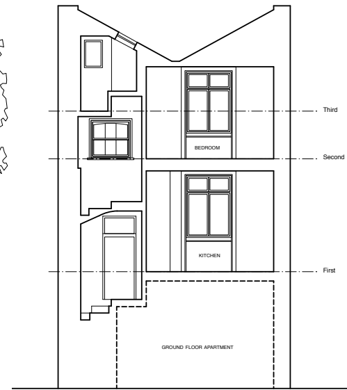
SHORT SECTION
