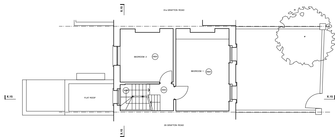
SECOND FLOOR
