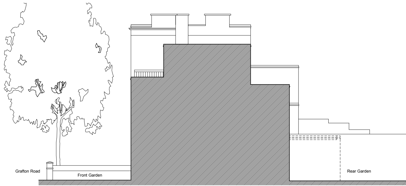
SIDE ELEVATION FROM 31a GRAFTON ROAD
