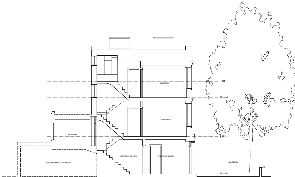
LONG SECTION
