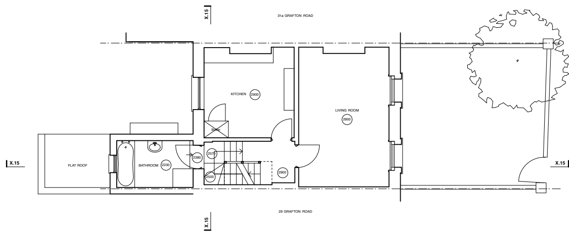
FIRST FLOOR
