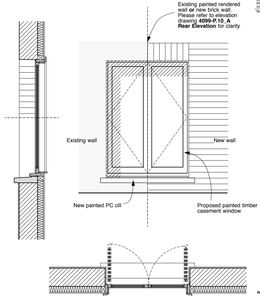
PROPOSED REAR WINDOW DETAILS - 1.20 SCALE
