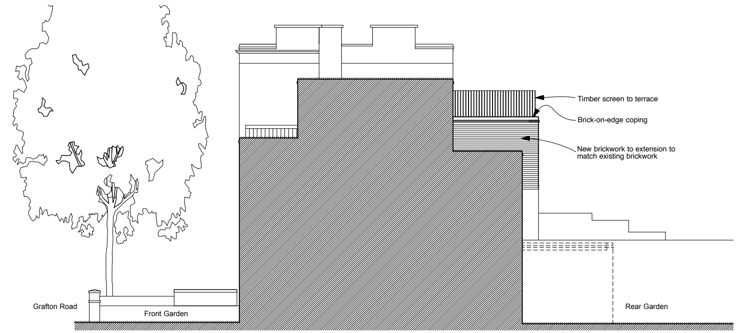
SIDE ELEVATION FROM 31a GRAFTON ROAD
