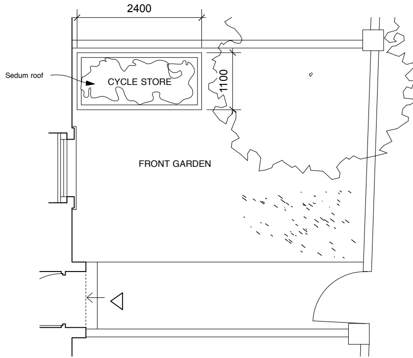
FRONT GARDEN PLAN
