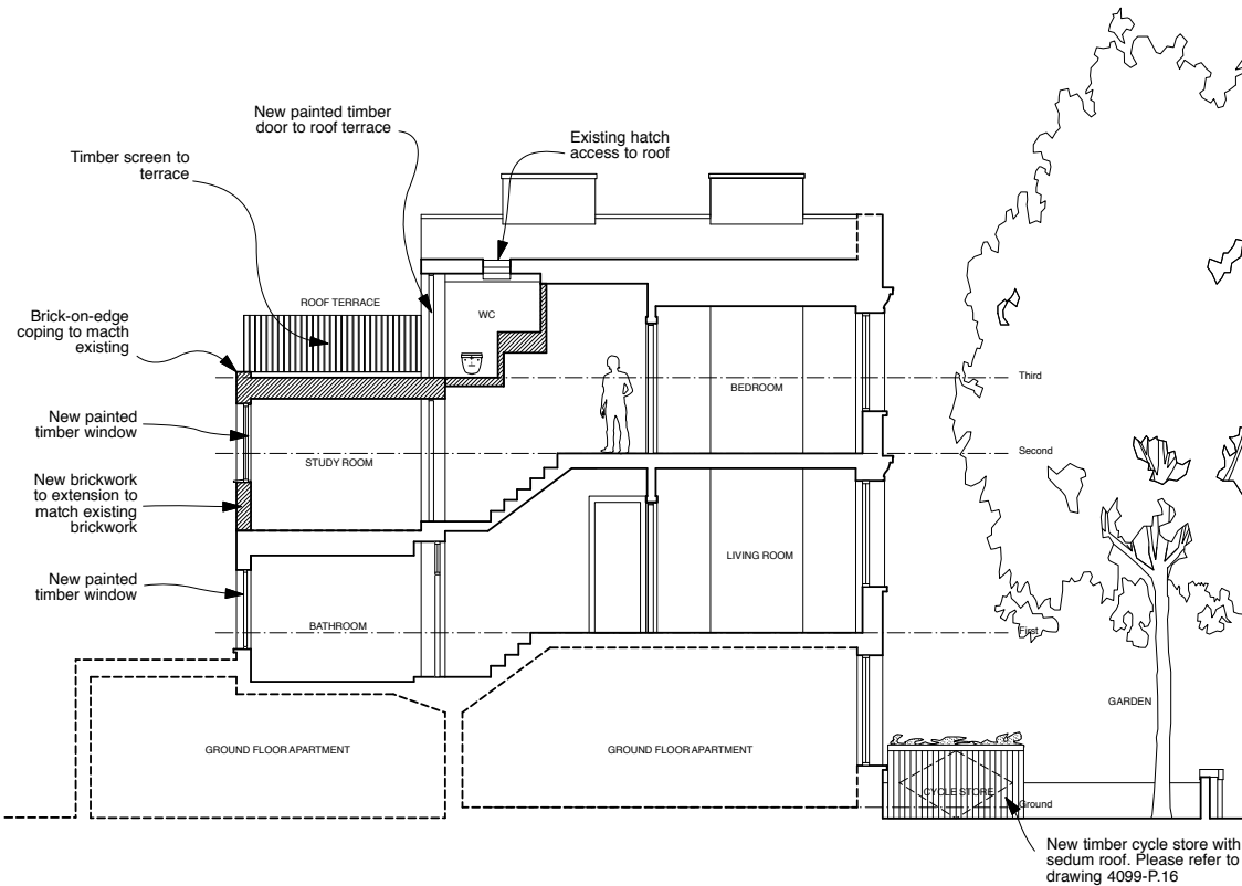
LONG SECTION
