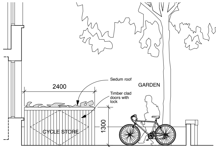
FRONT GARDEN SECTION
