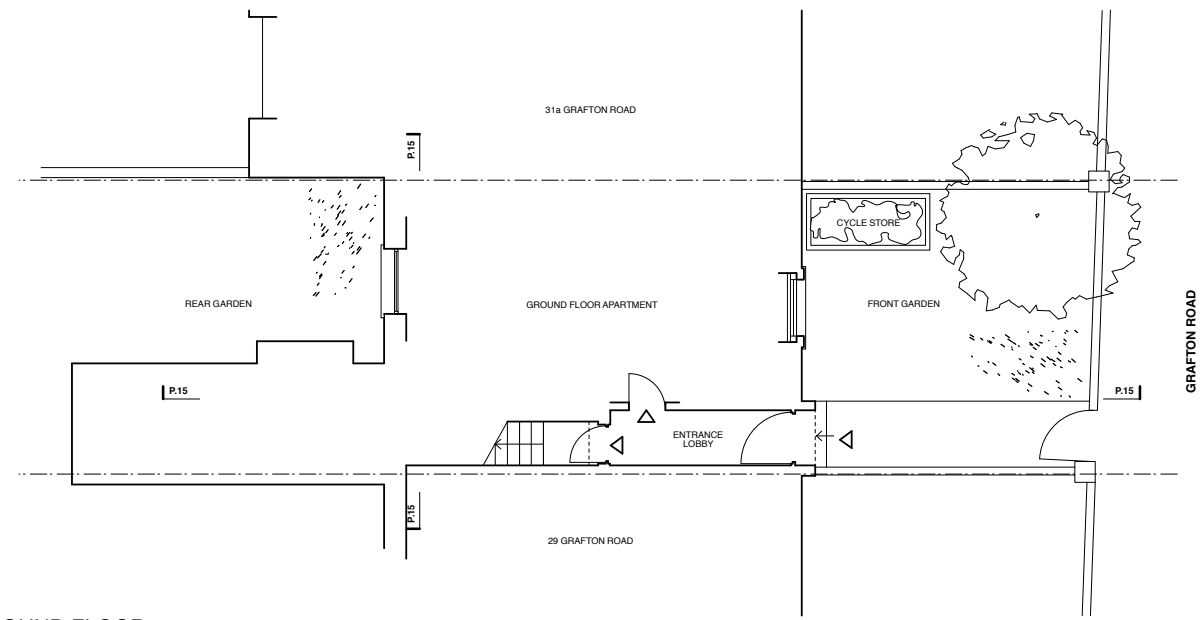
GROUND FLOOR
