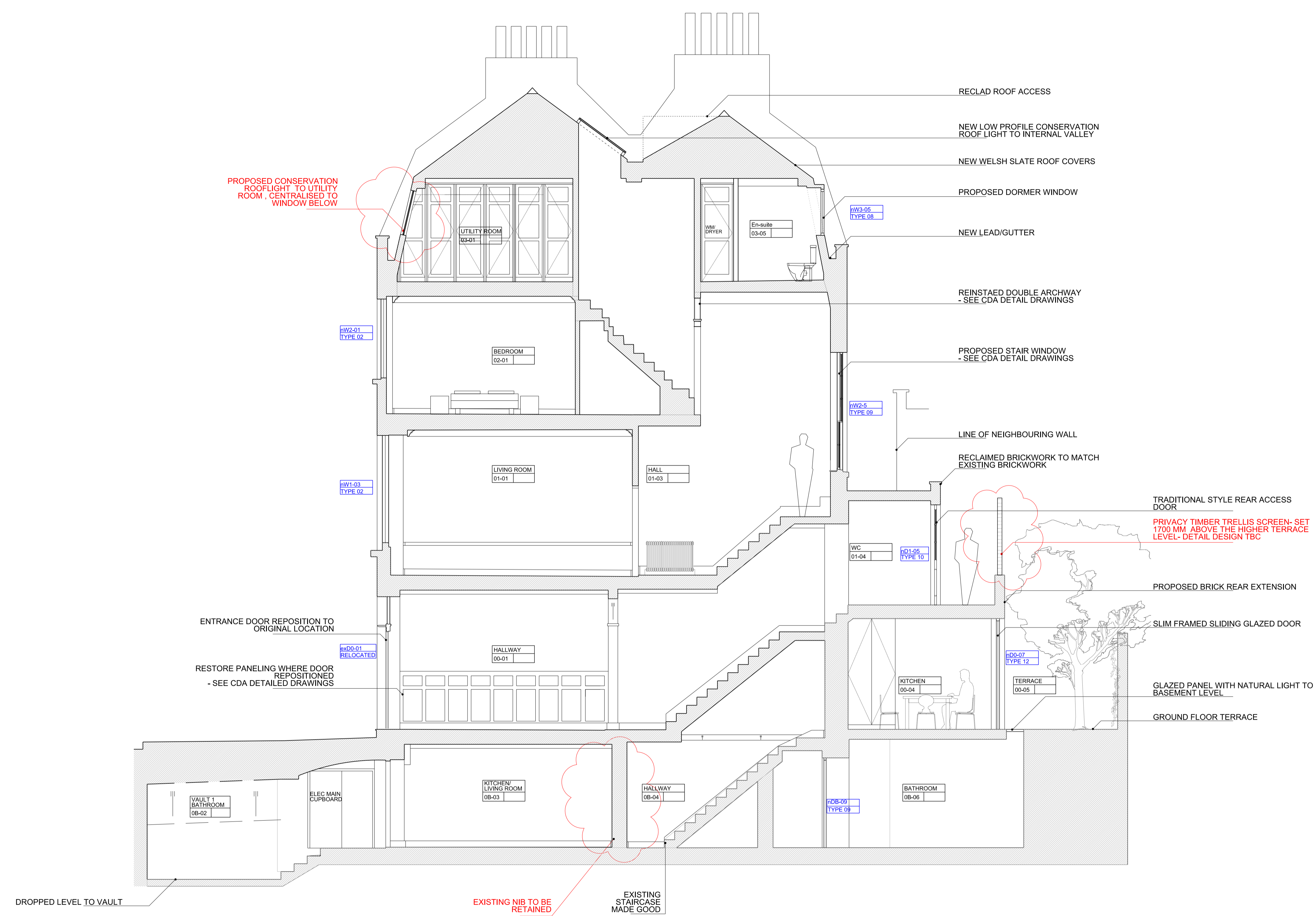
1 1:50 / 1:100 PROPOSED SECTION A
