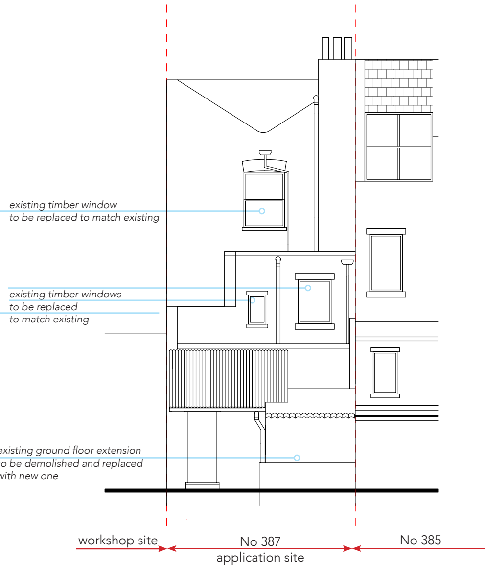
Existing Rear Elevation (B)
