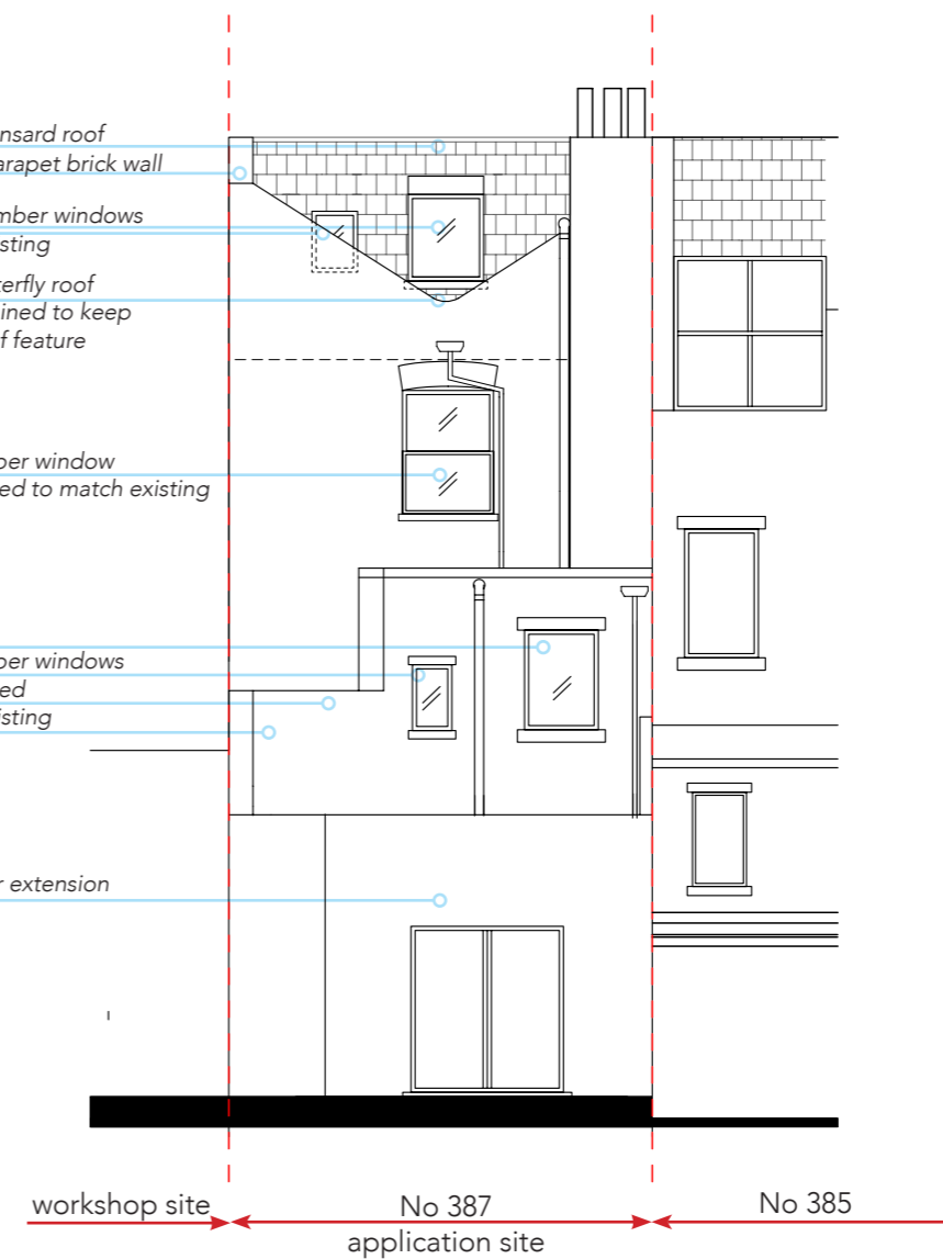
Proposed Rear Elevation (Section B)
