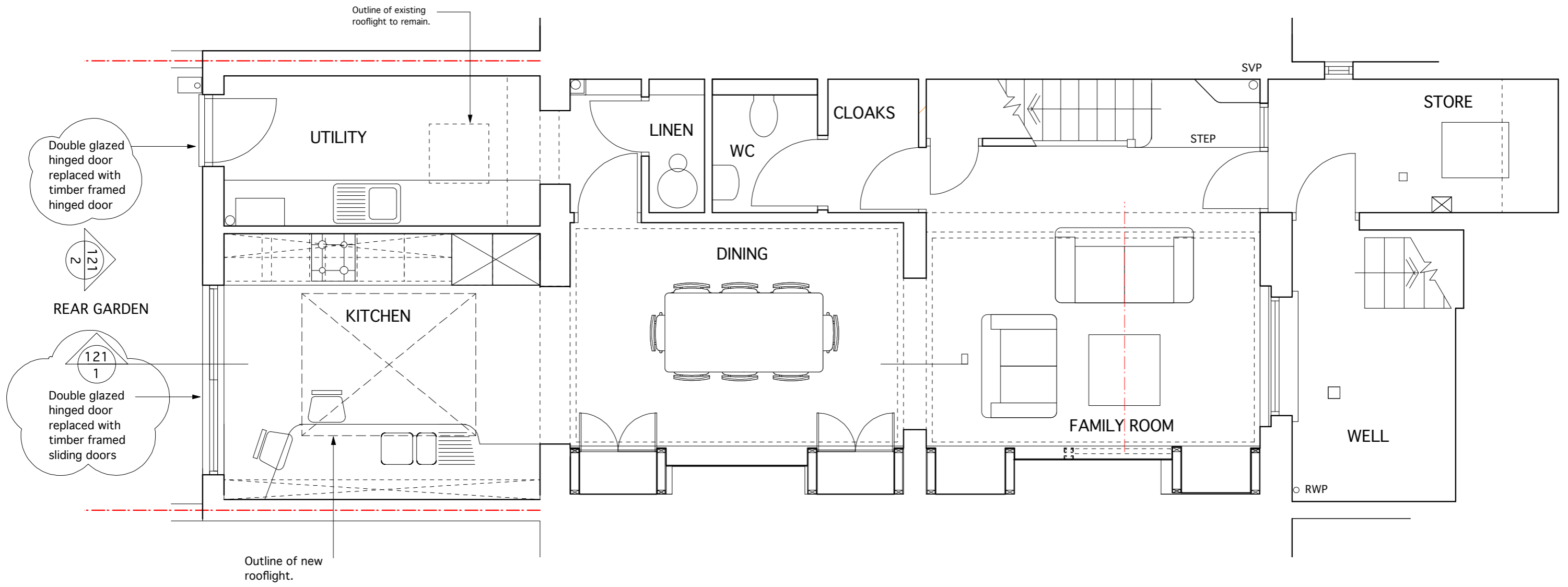
1 PROPOSED LOWER GROUND PLAN SCALE 1:50
