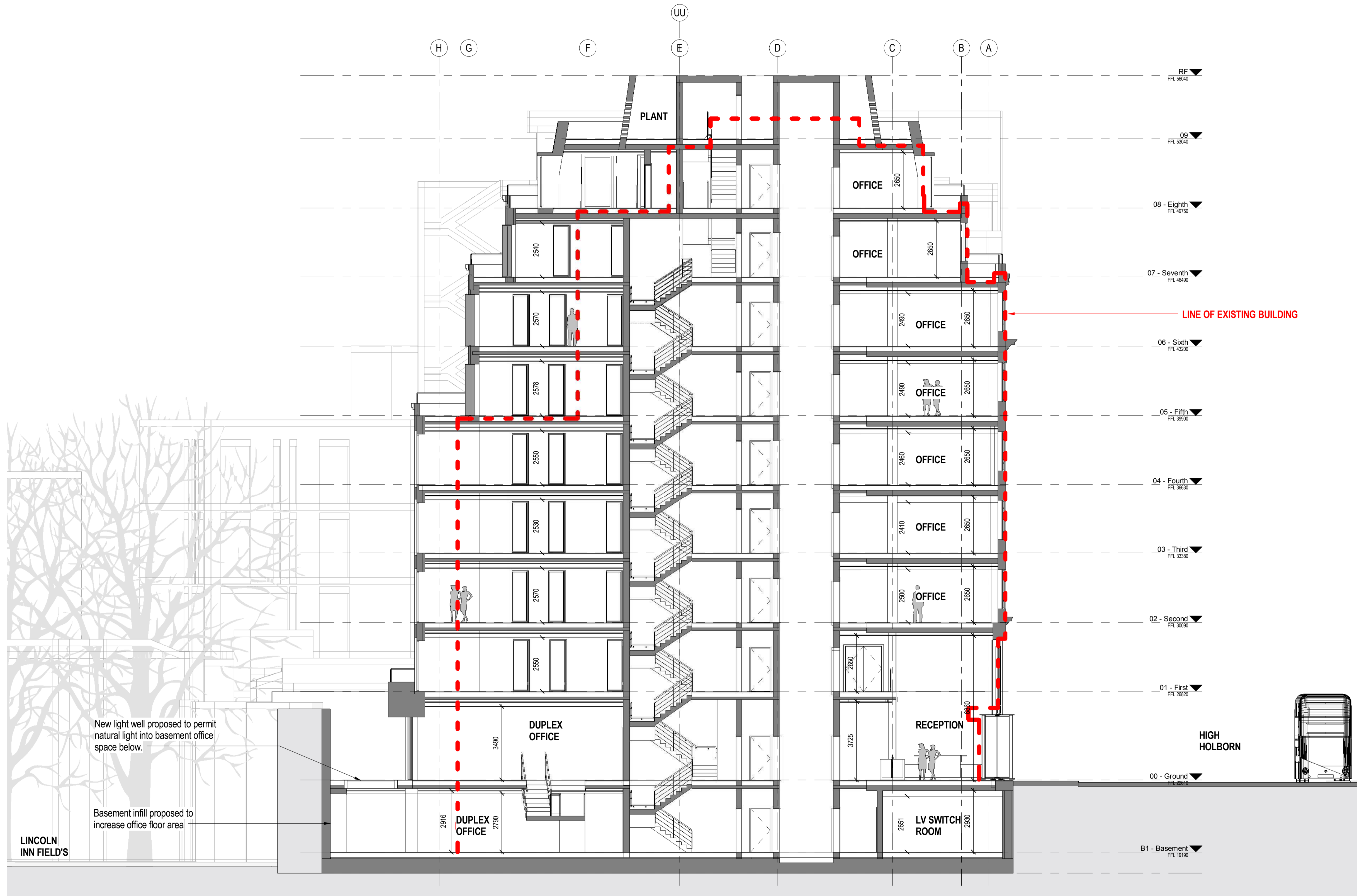
1 0239 521-Section-A-A 1:100
