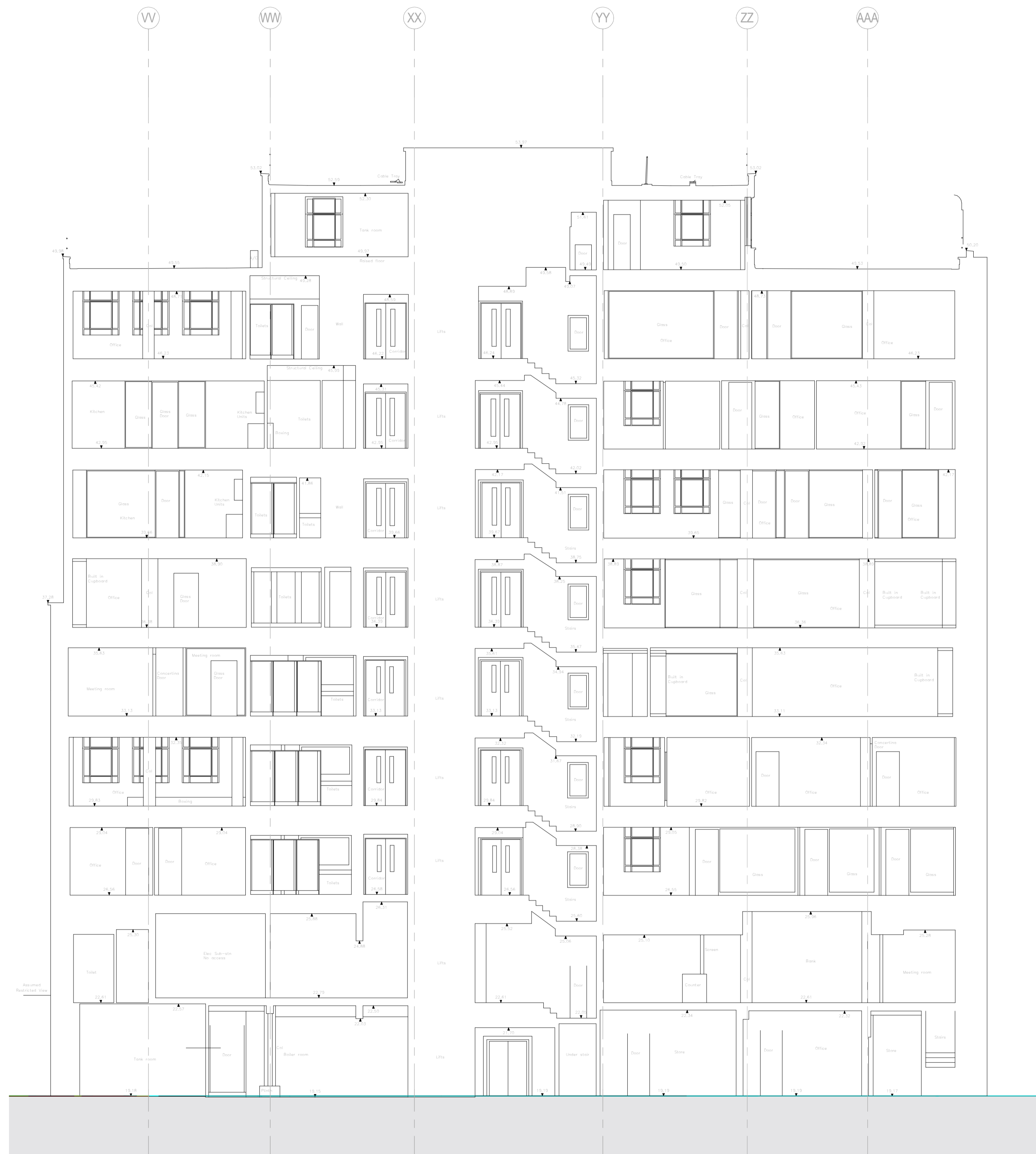
1 502-Section B-B 1:100
