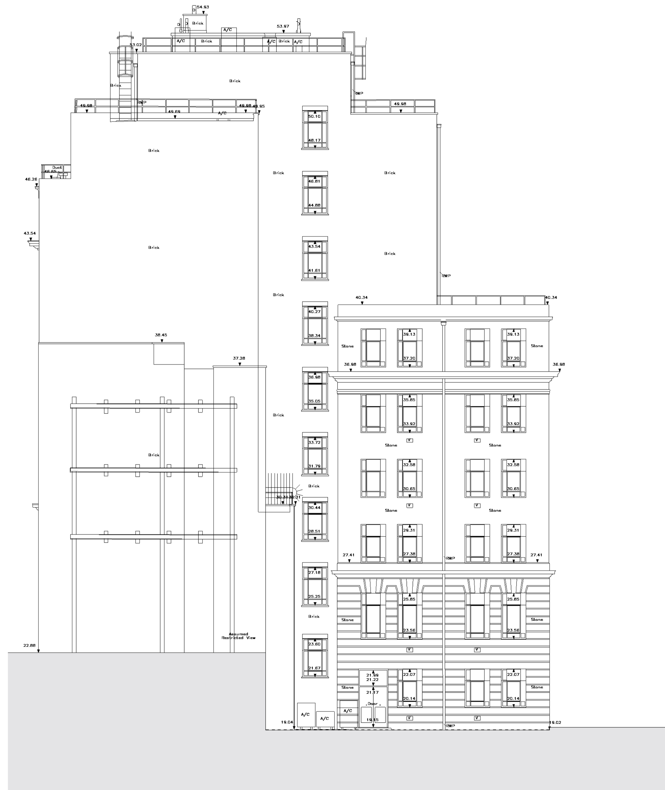
1 0402-WE-Existing Elevation 1:100
