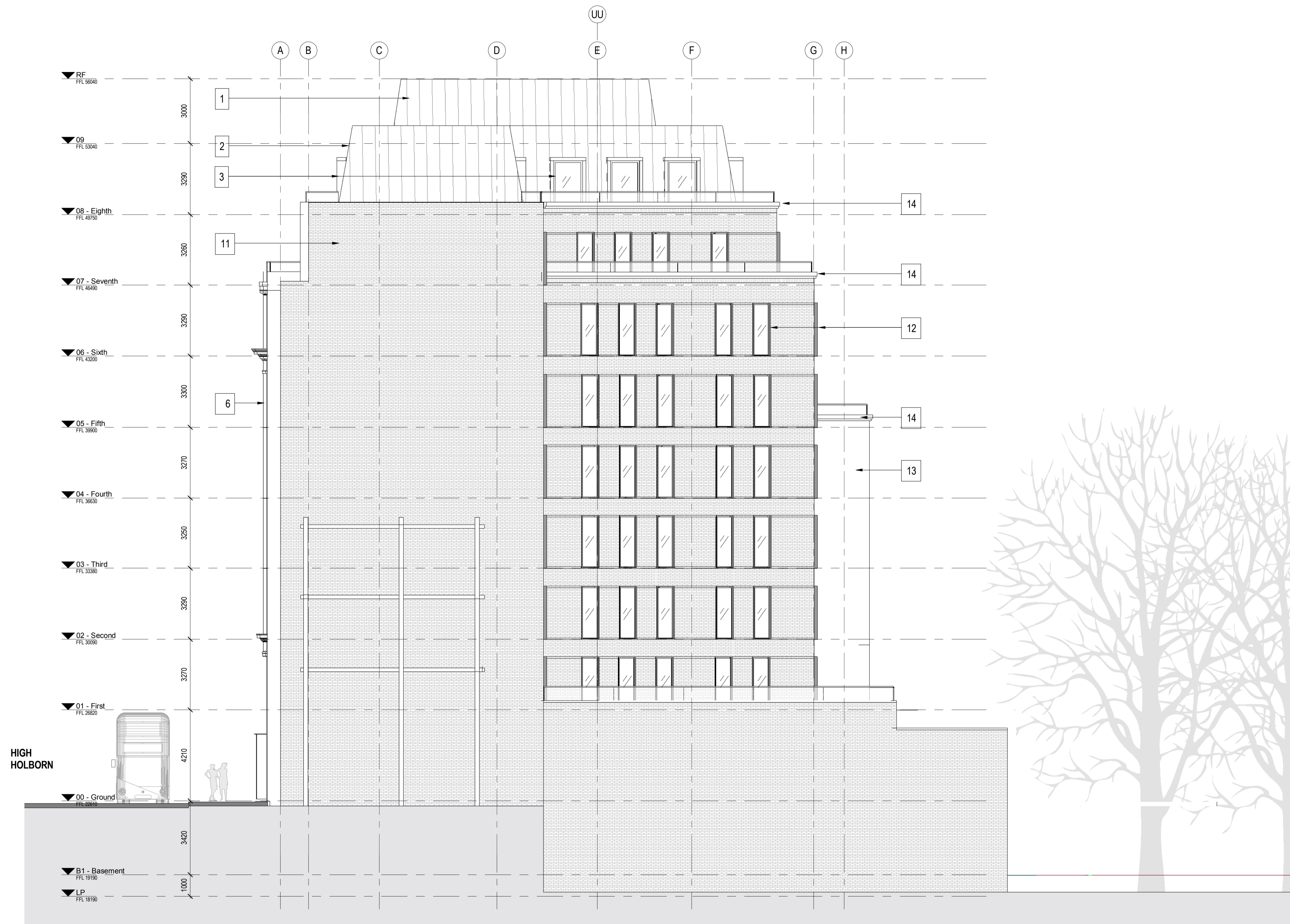
1 0422-WE-Elevation 1:100
