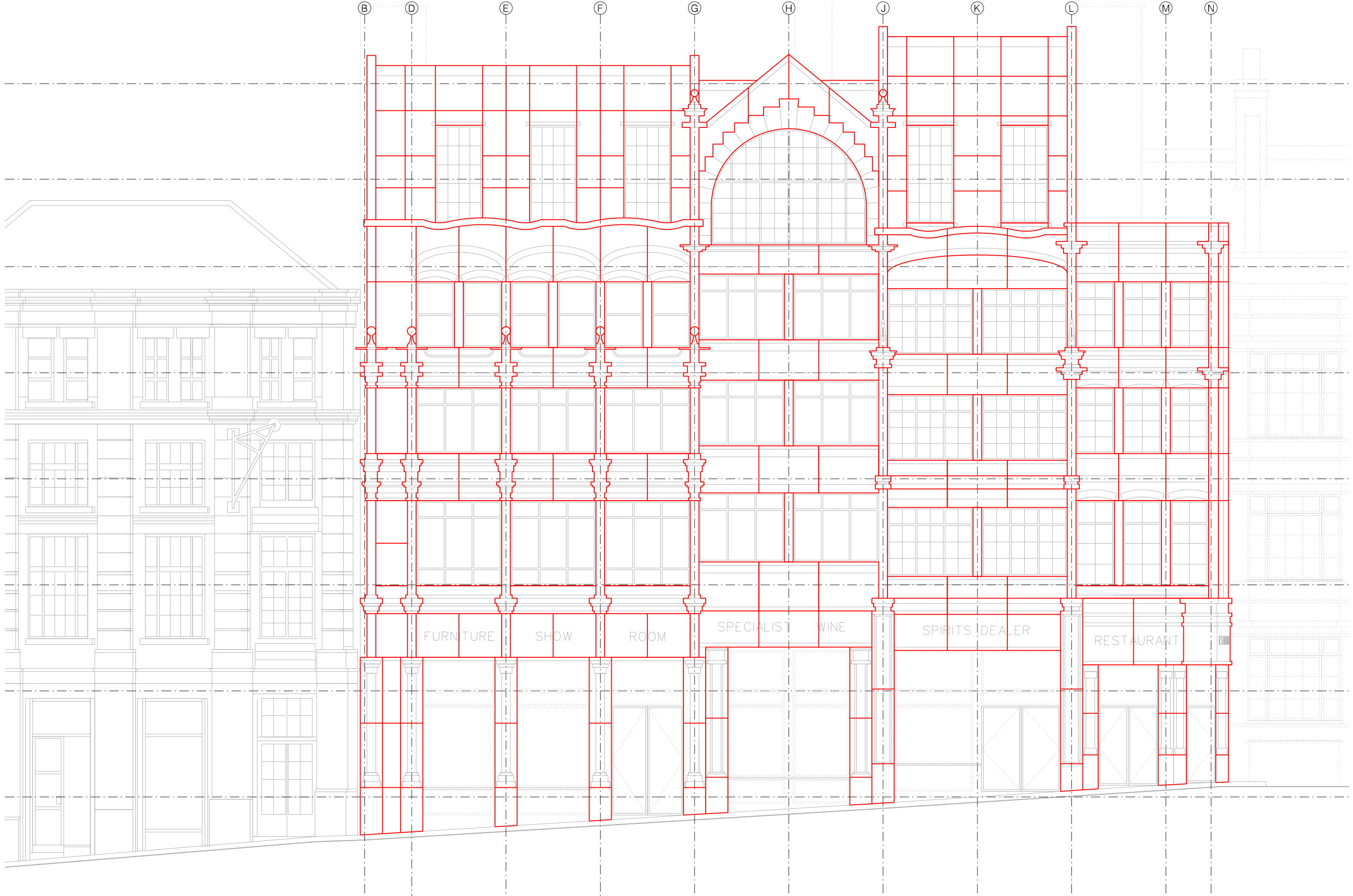
① PROPOSED NORTH ELEVATION – PANEL SUBDIVISION
