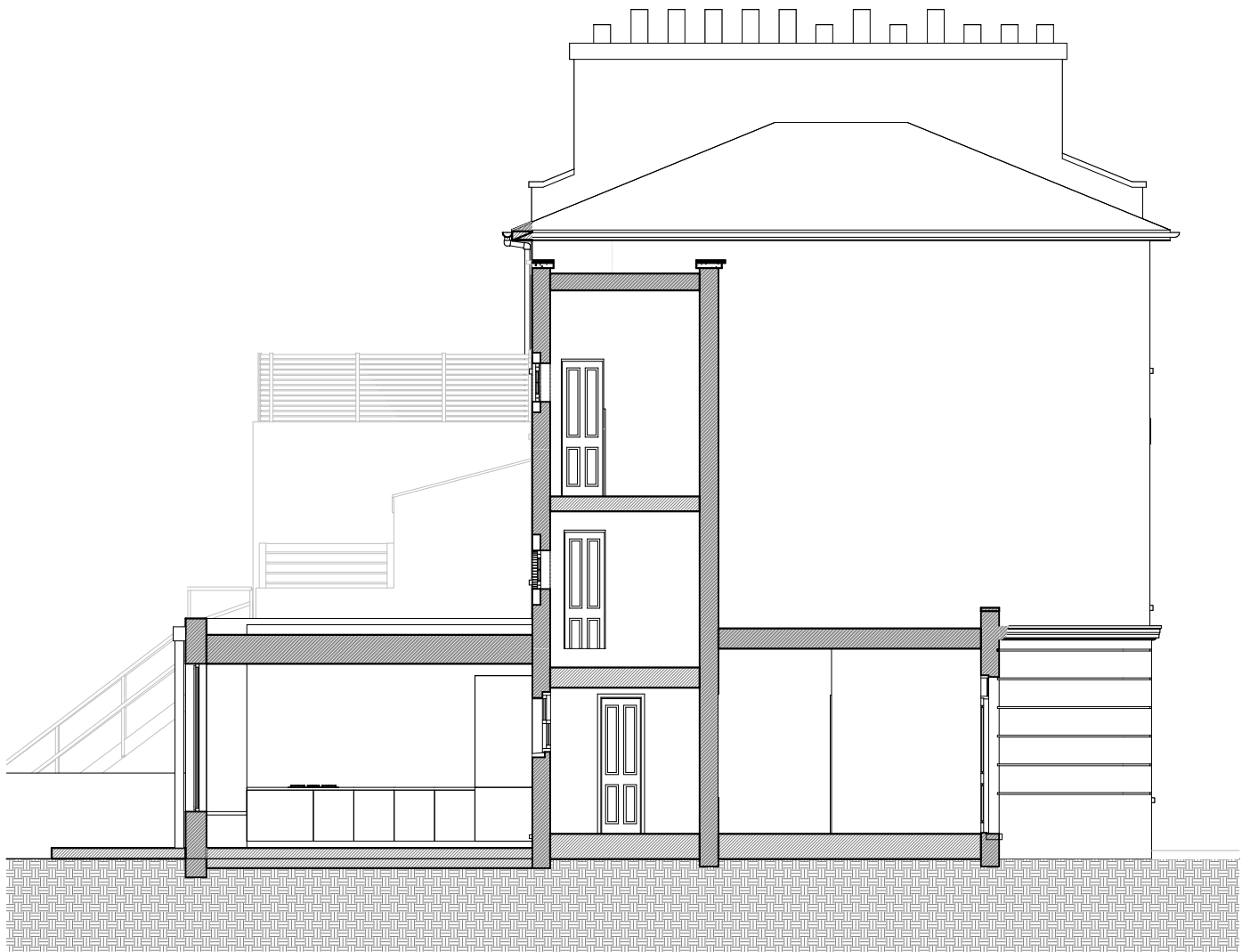
B-B - EXISTING BUILDING SECTION SCALE: 1:100@A3
