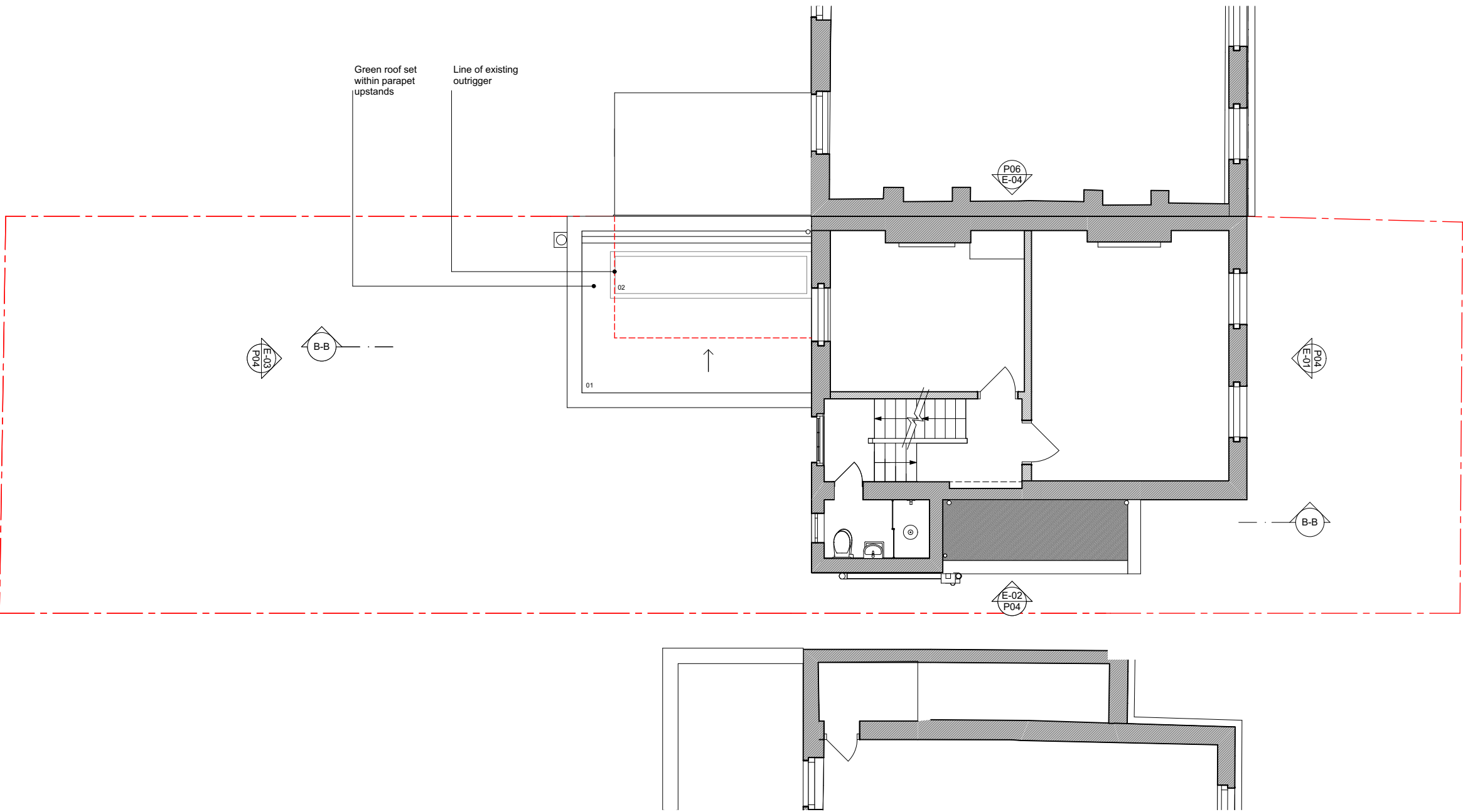
PROPOSED FIRST FLOOR PLAN PD - FPA REAR SCALE: 1:100@A3
