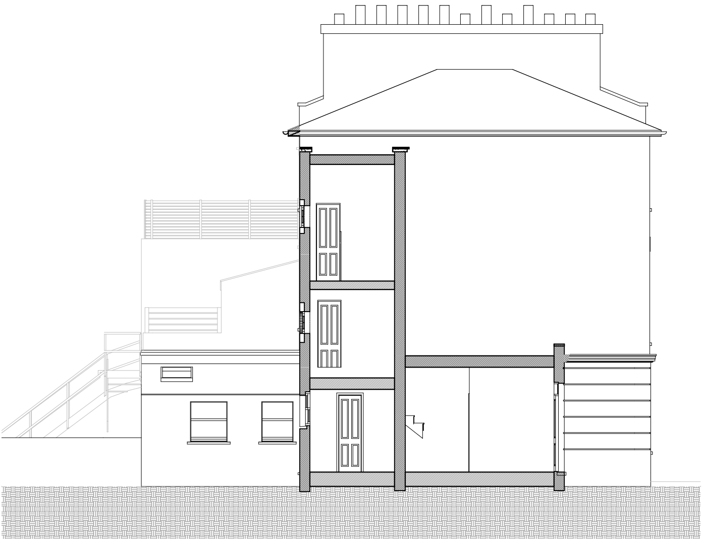
EXISTING BUILDING SECTION SCALE: 1:100@A3
