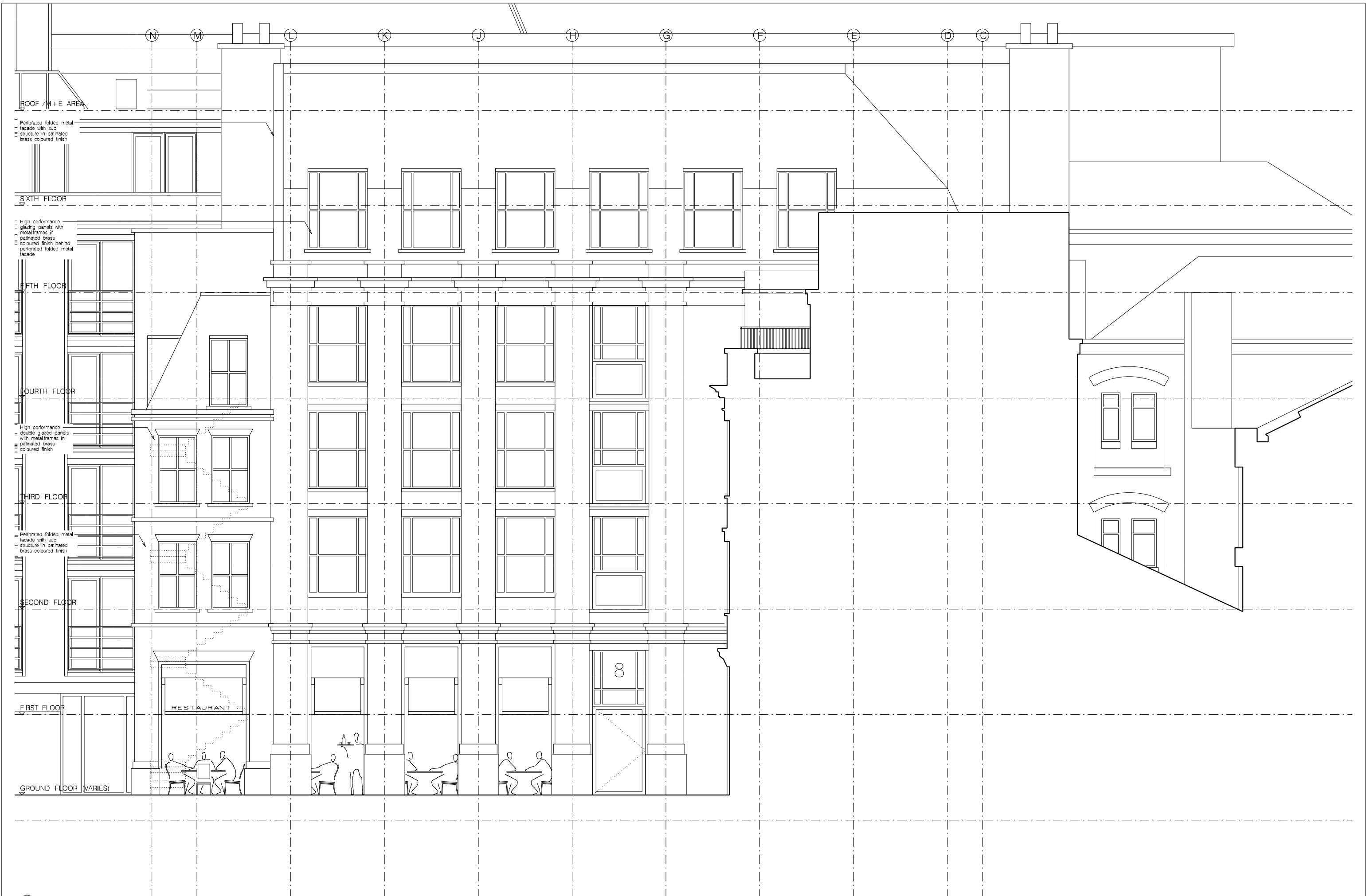
① PROPOSED SOUTH ELEVATION
