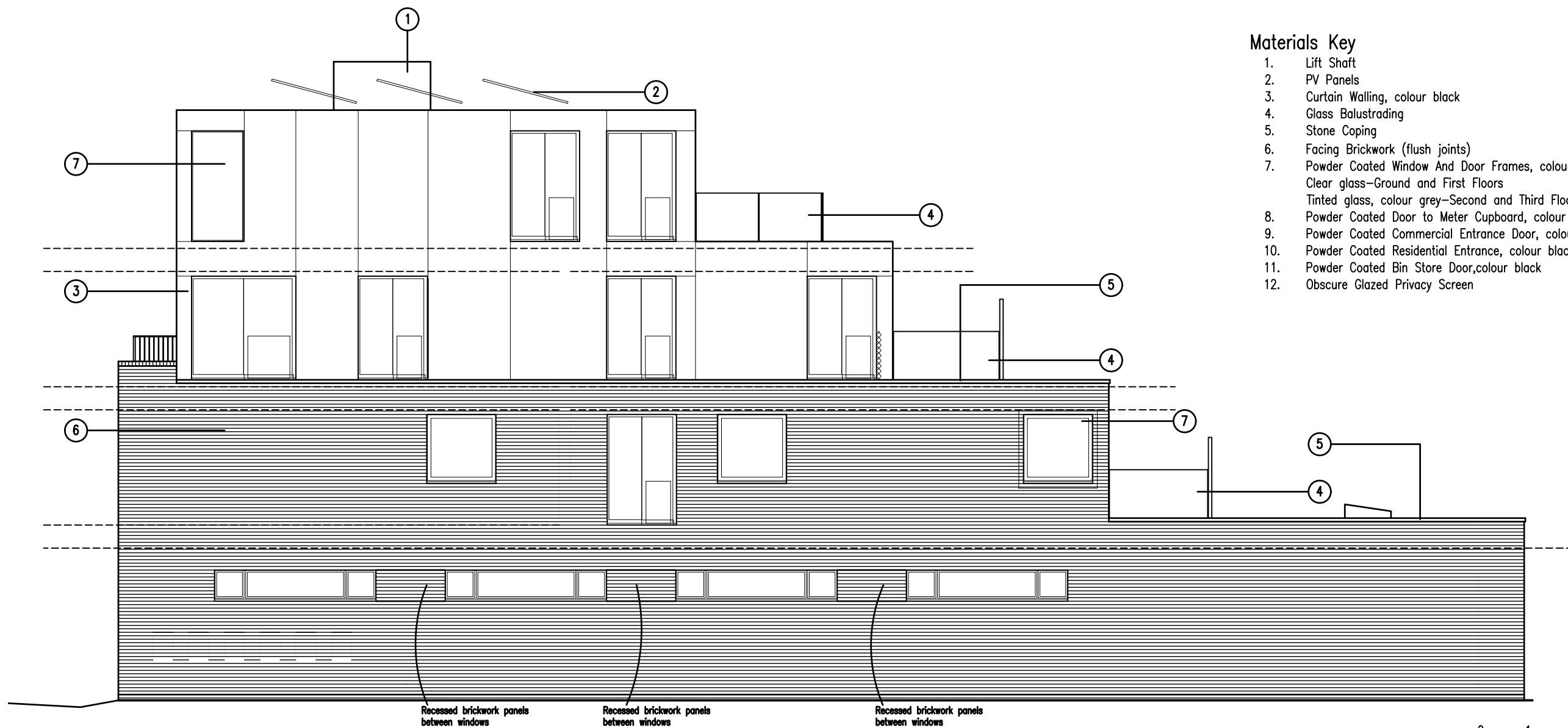
Side Elevation
