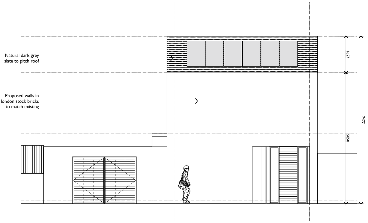
01 ENTRY (SOUTH) ELEVATION, ALONG ROCHESTER MEWS
