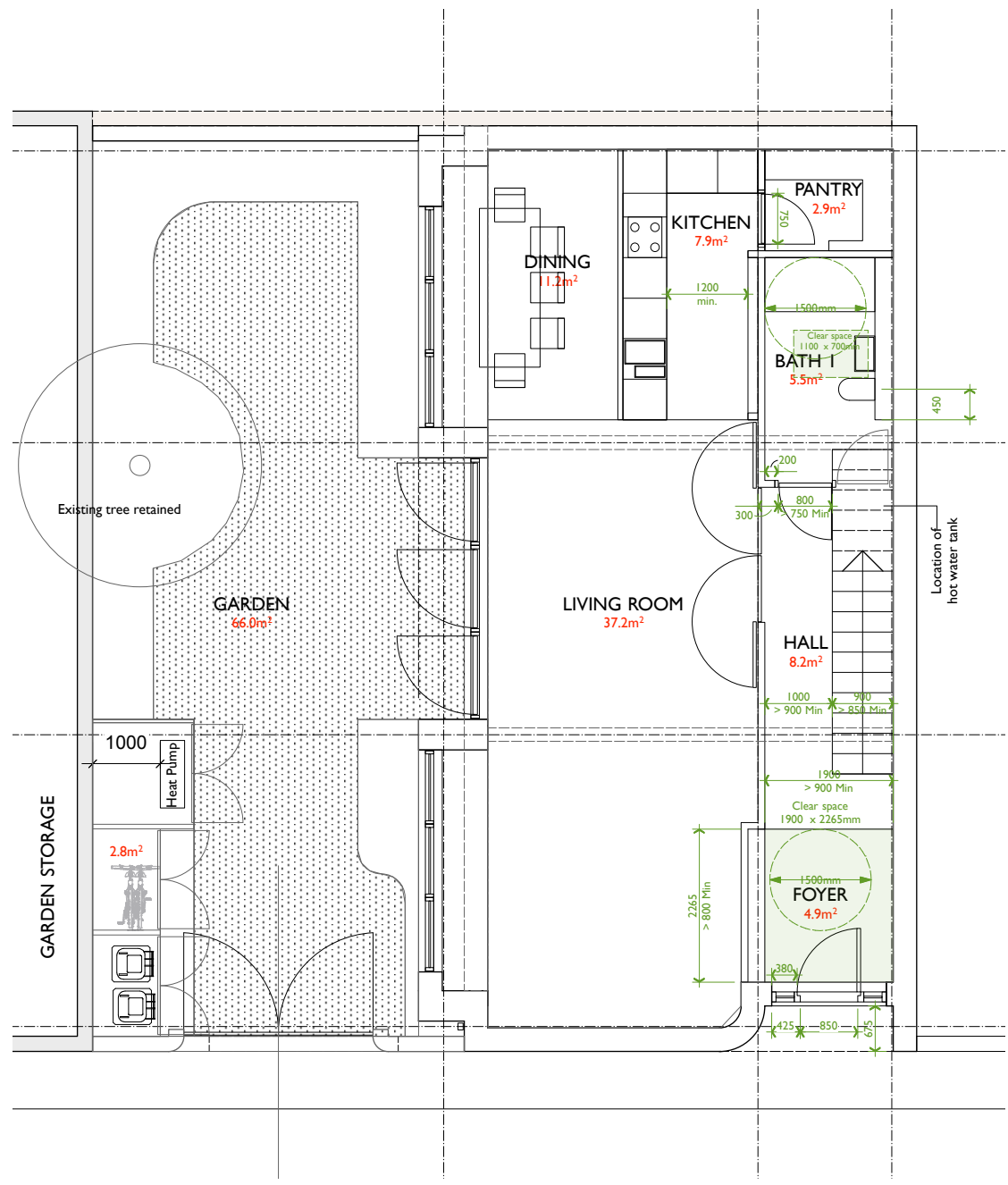
01 GROUND FLOOR PLAN
