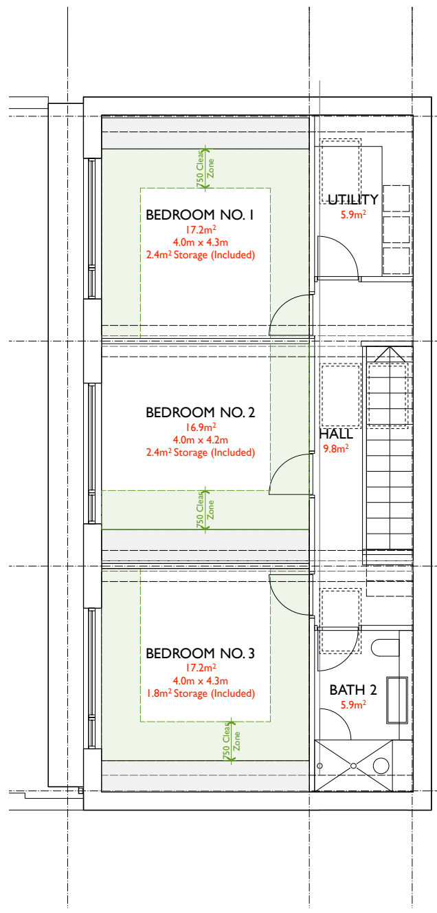
02 FIRST FLOOR PLAN
