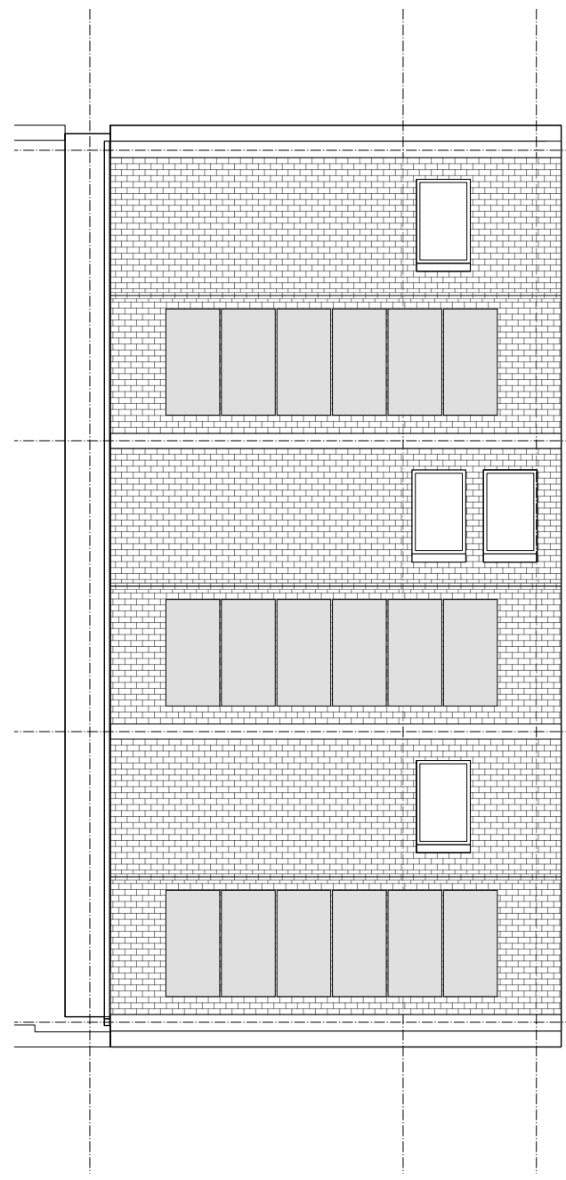
03 ROOF PLAN
