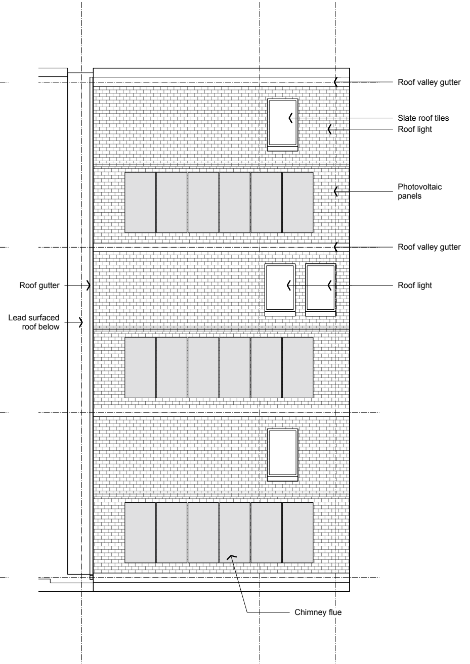
03 ROOF PLAN
