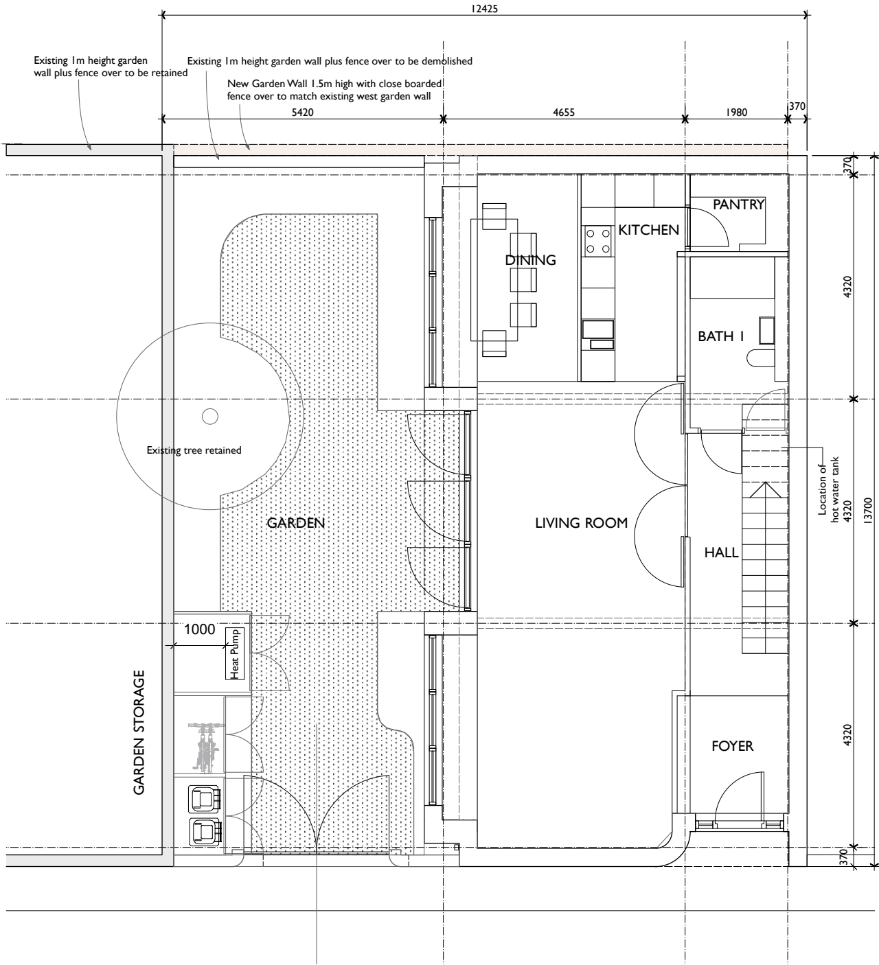
01 GROUND FLOOR PLAN
