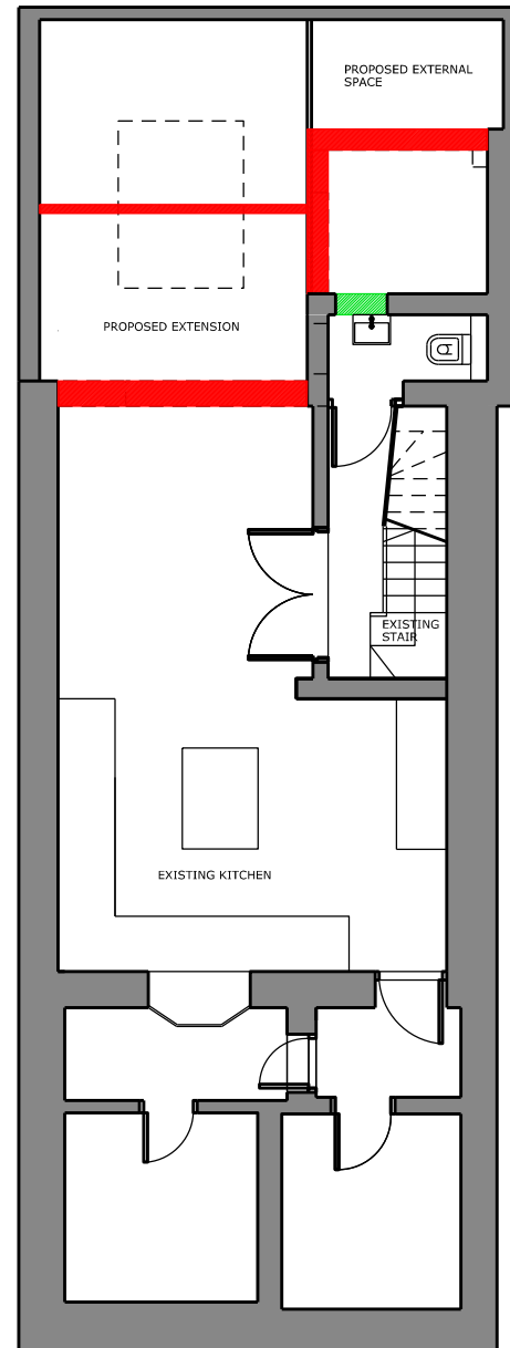
LOWER GROUND FLOOR - PROPOSED
