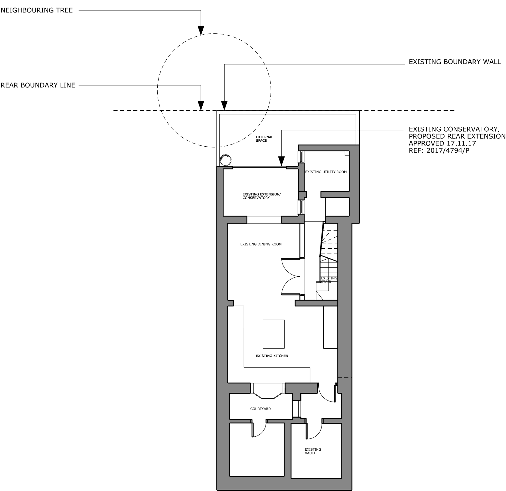
LOWER GROUND FLOOR - EXISTING
