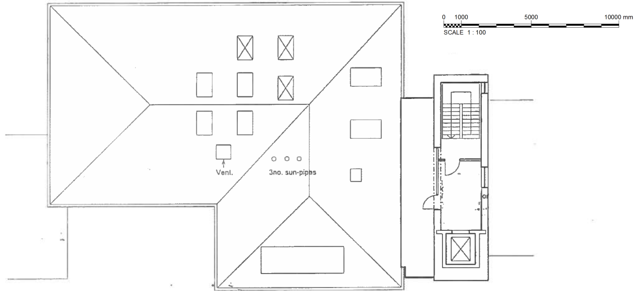
FIRST FLOOR AND PART ROOF
