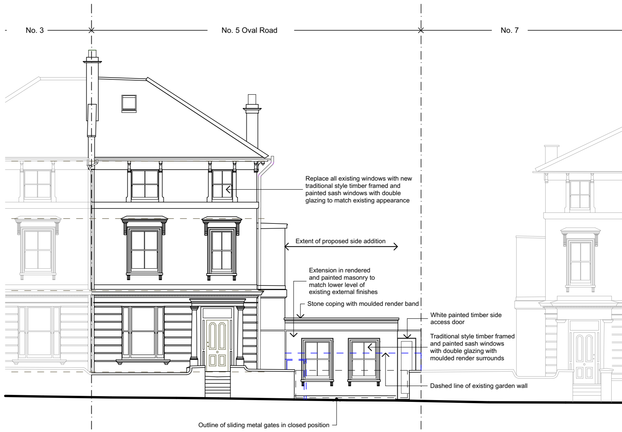
PROPOSED - NORTH EAST ELEVATION
