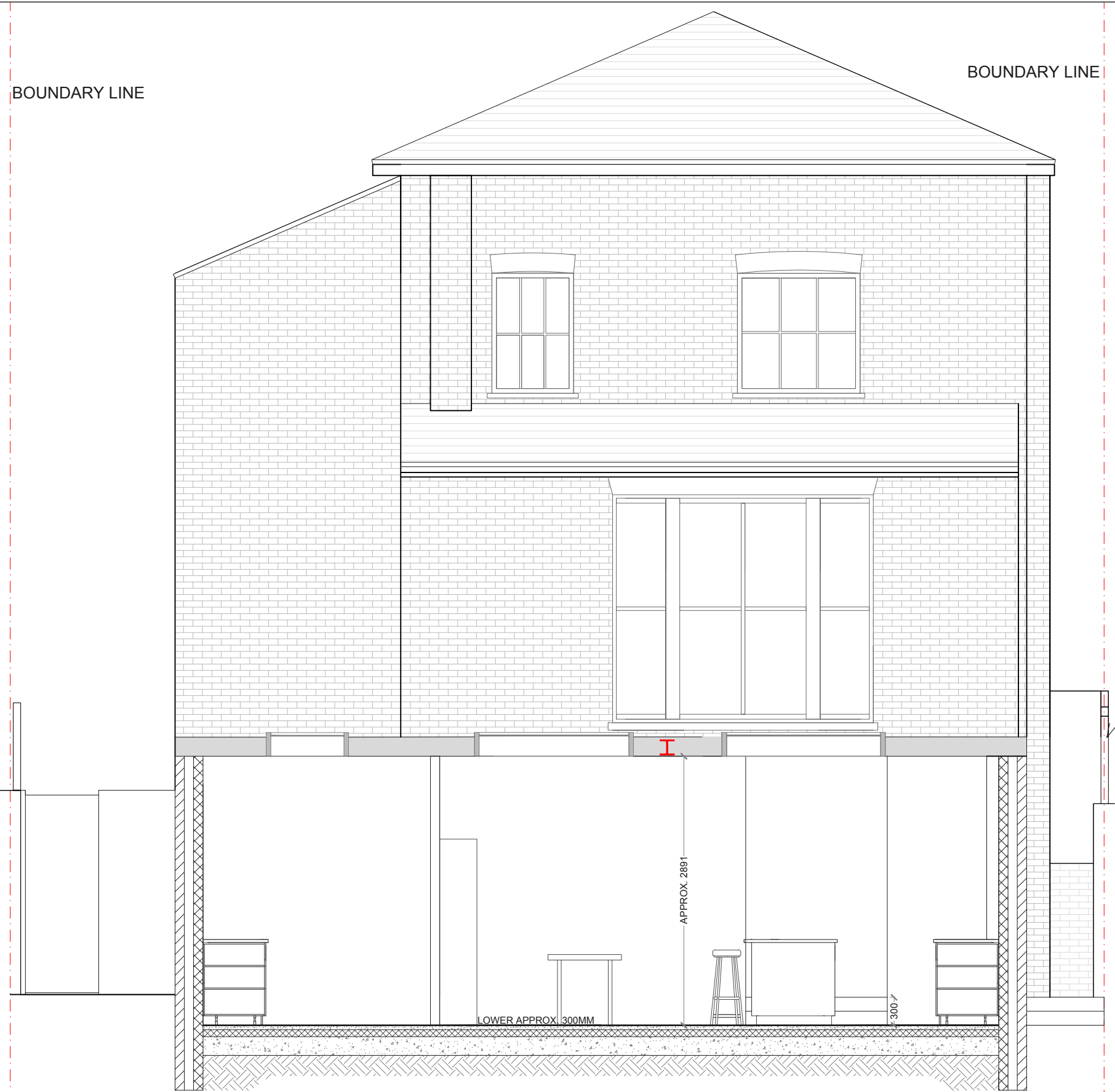
PROPOSED SECTION AA SCALE 1:50
