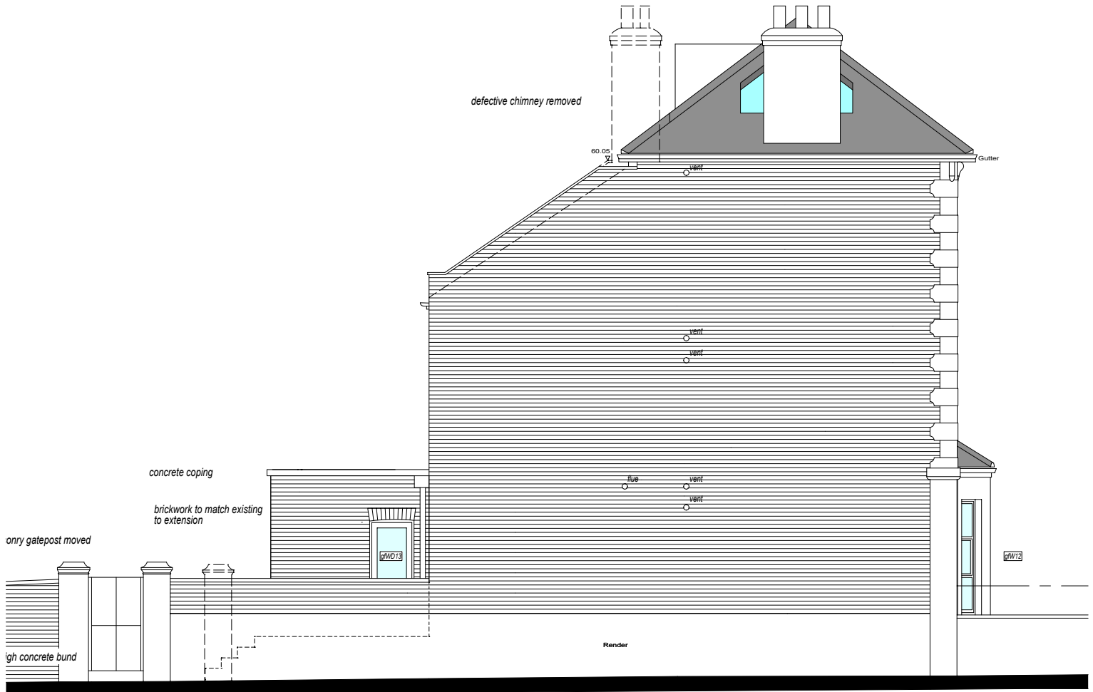
ELEVATION TO YORK RISE - SW
