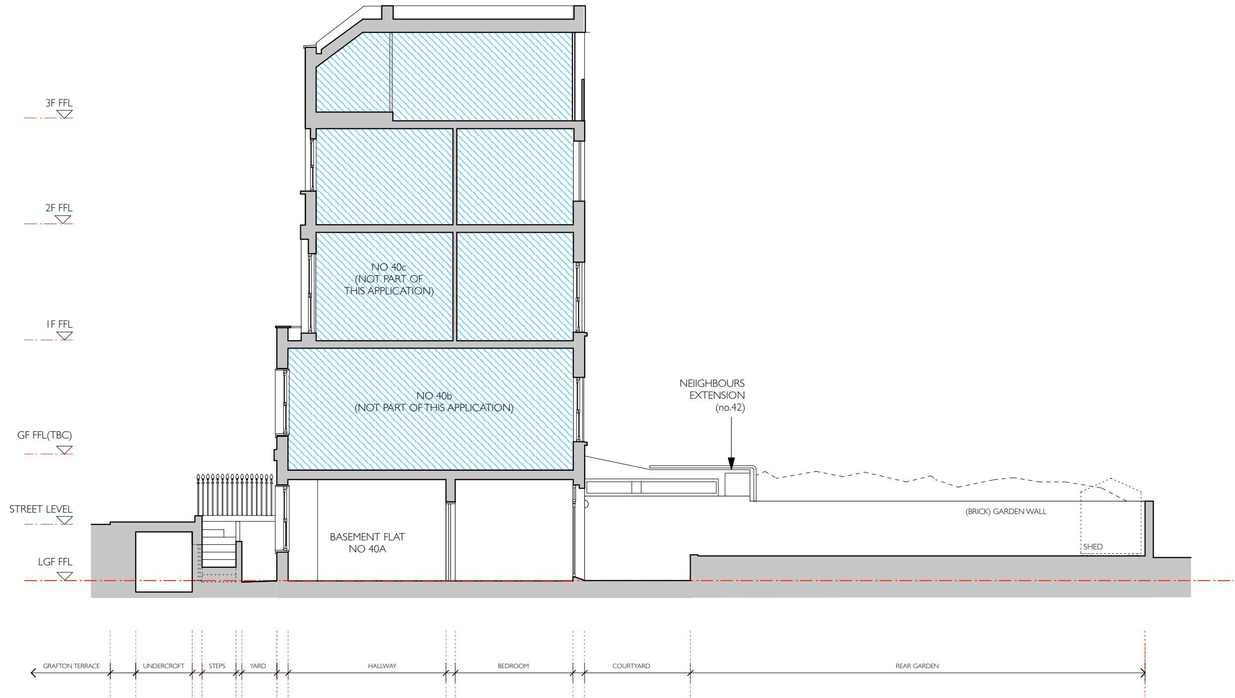
A EXISTING SECTION B - B SCALE 1:100
