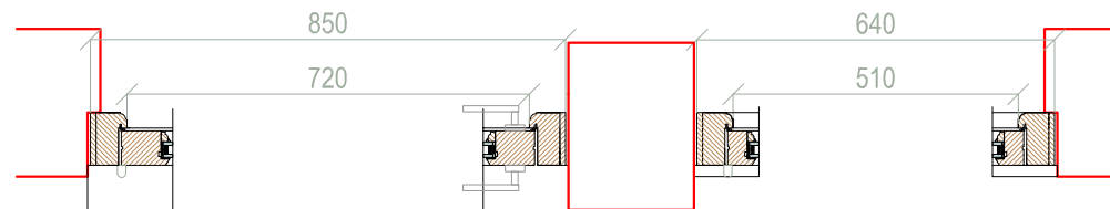
PLAN SECTION
