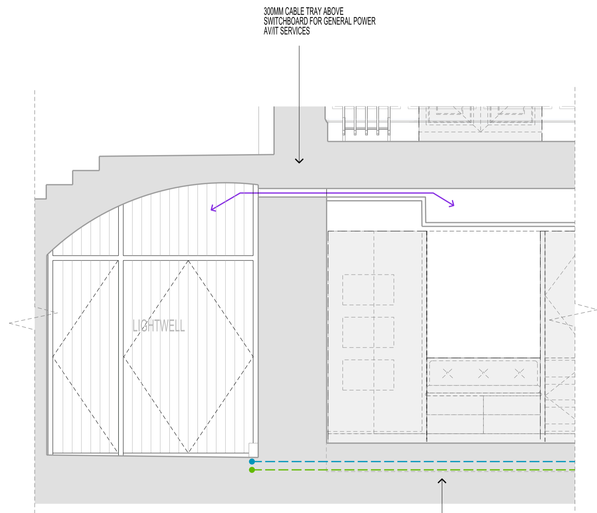
Section A_A Scale 1:25 at A1
