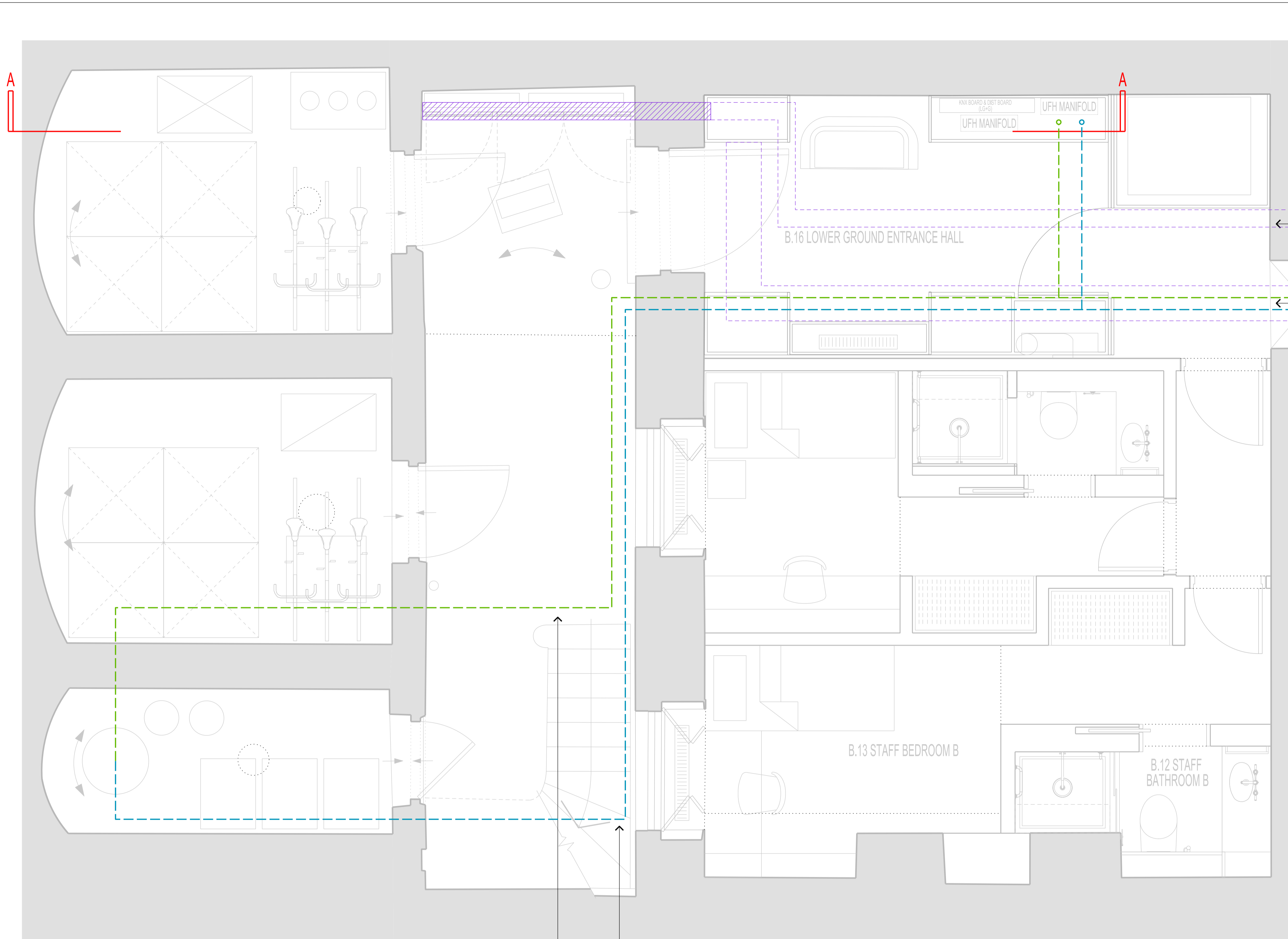
Lower Ground Floor Plan Scale 1:25 at A1
