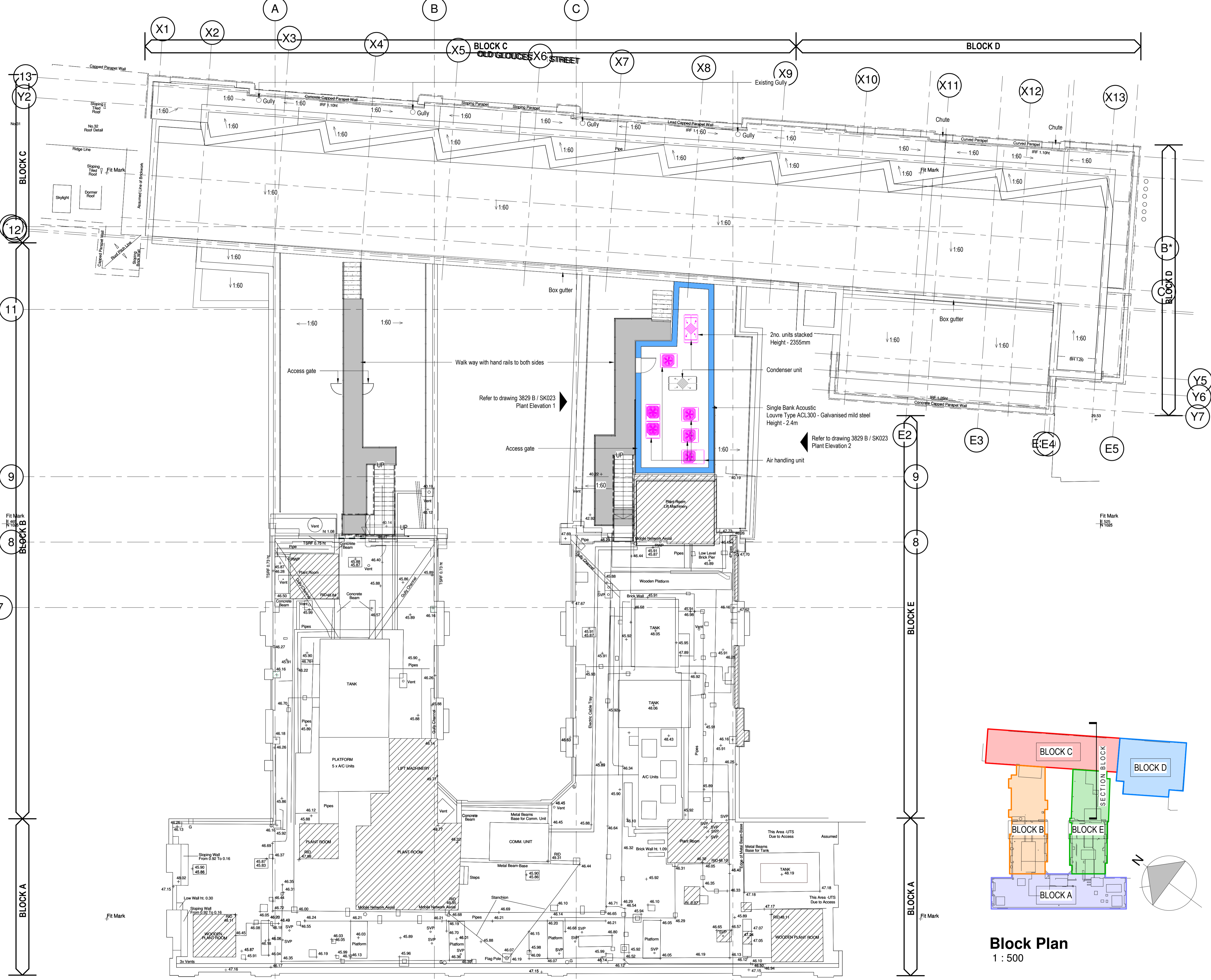
Proposed Plant Layout 1 : 100
