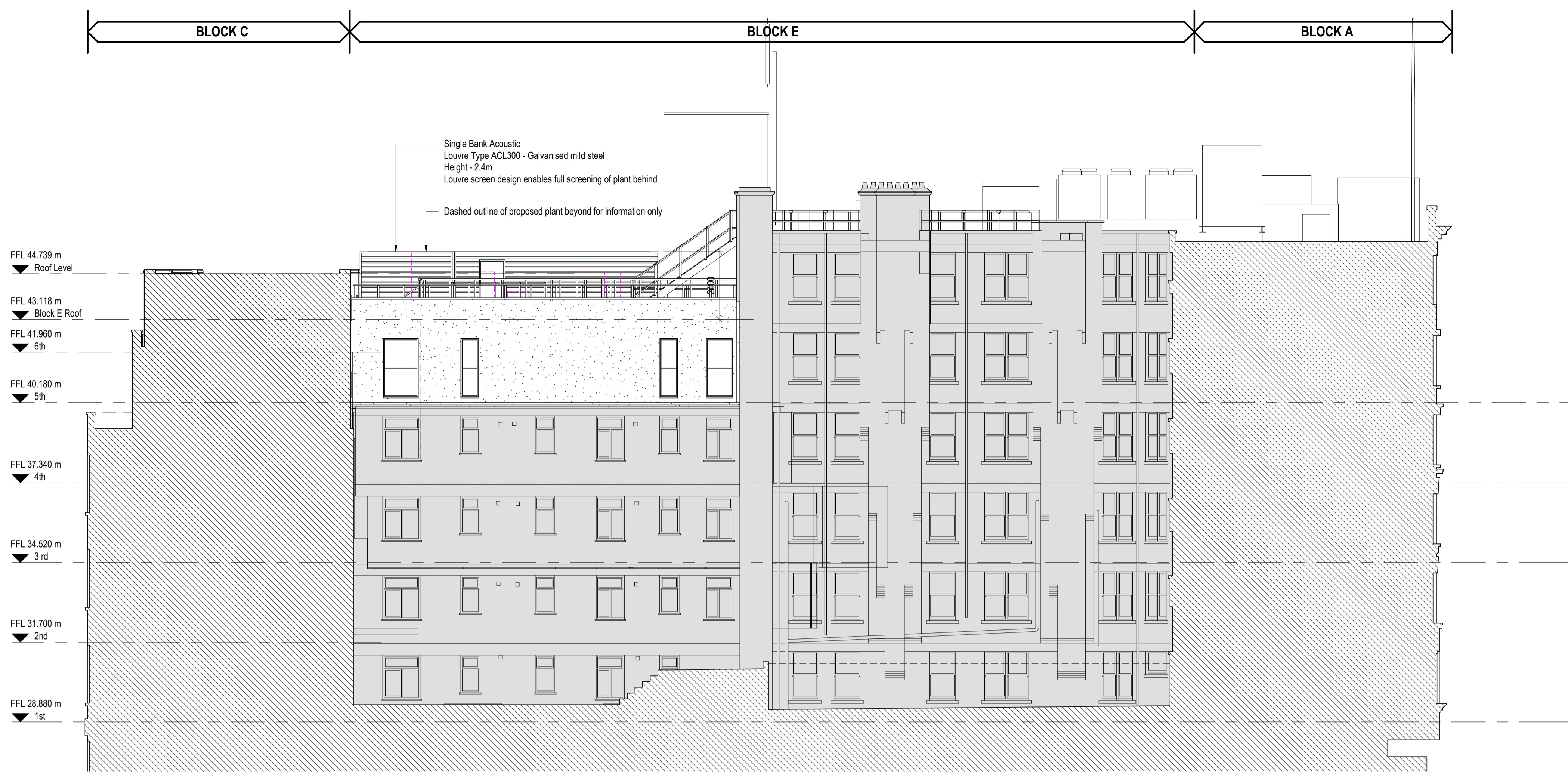
Plant Elevation 1 1 : 100
