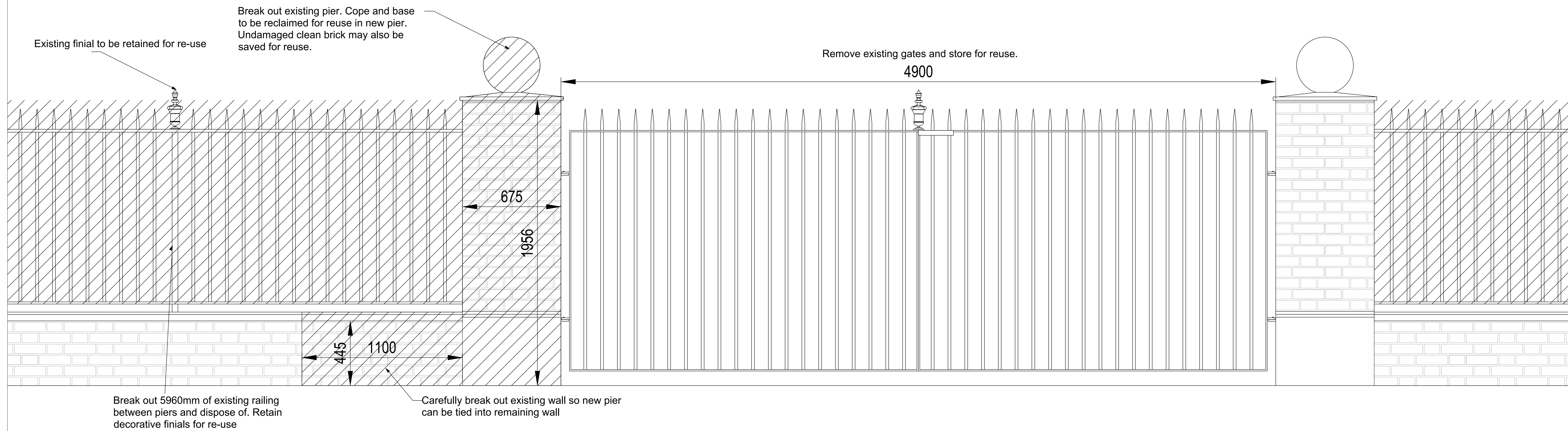
Existing Vehicular Entrance Gates - Demolition Scale 1:10
