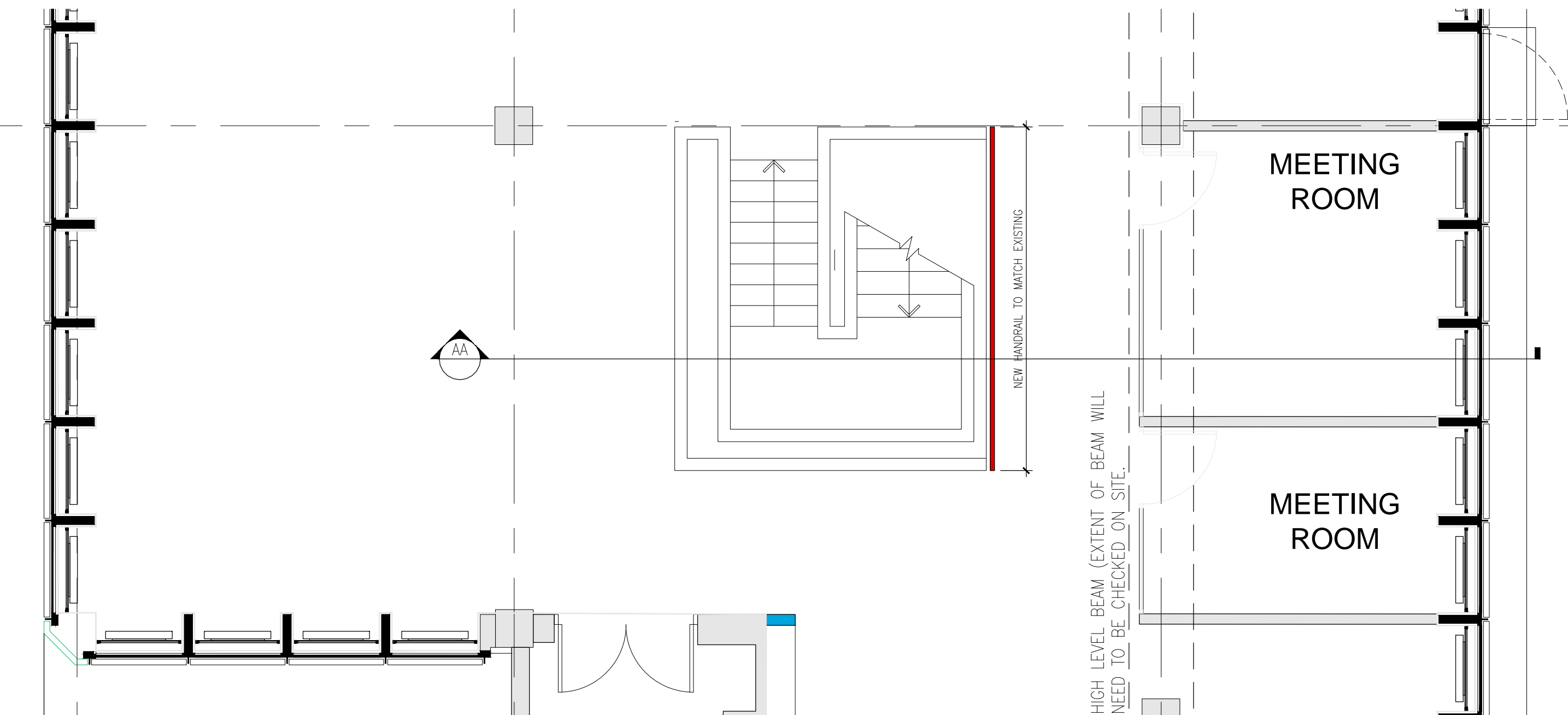
1 LEVEL 5 WING PART PLAN SCALE 1:50
