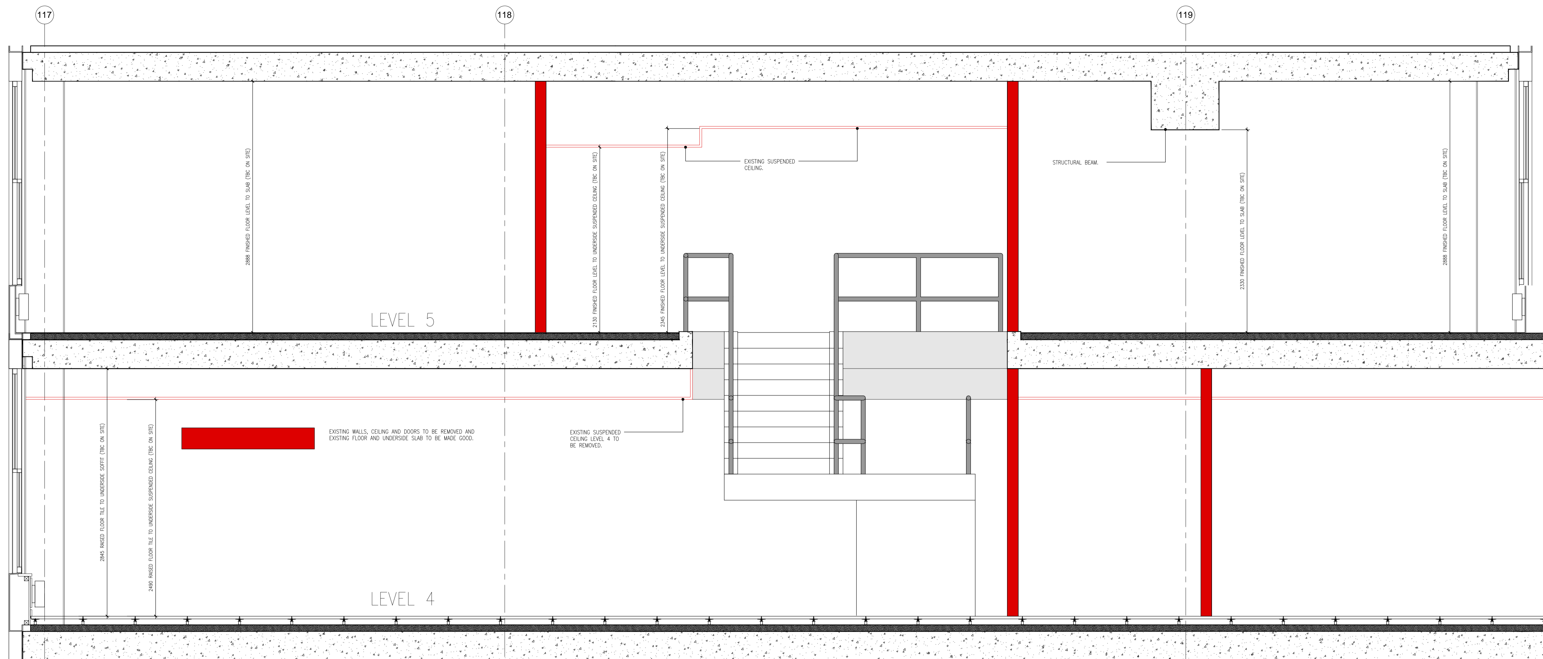
AA EXISTING PART SECTION THROUGH LEVEL 5 WING & STAIR SCALE 1:20
