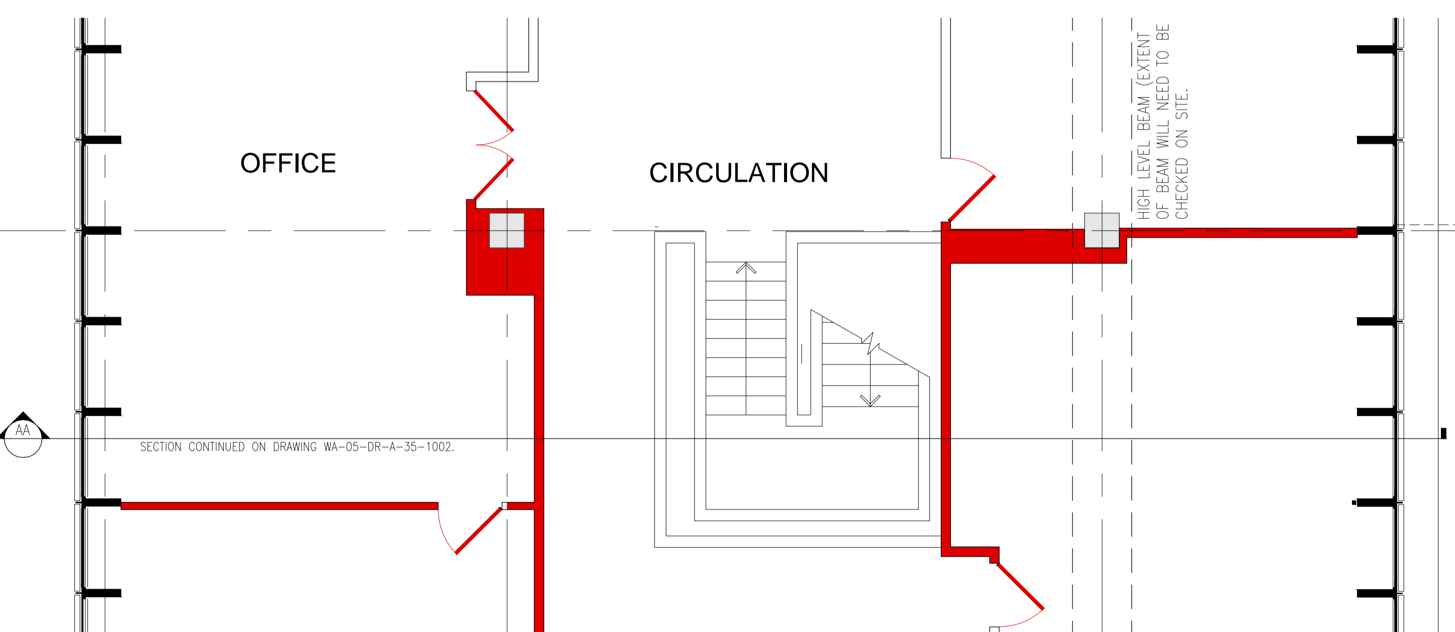
1 LEVEL 5 WING PART PLAN SCALE 1:50
