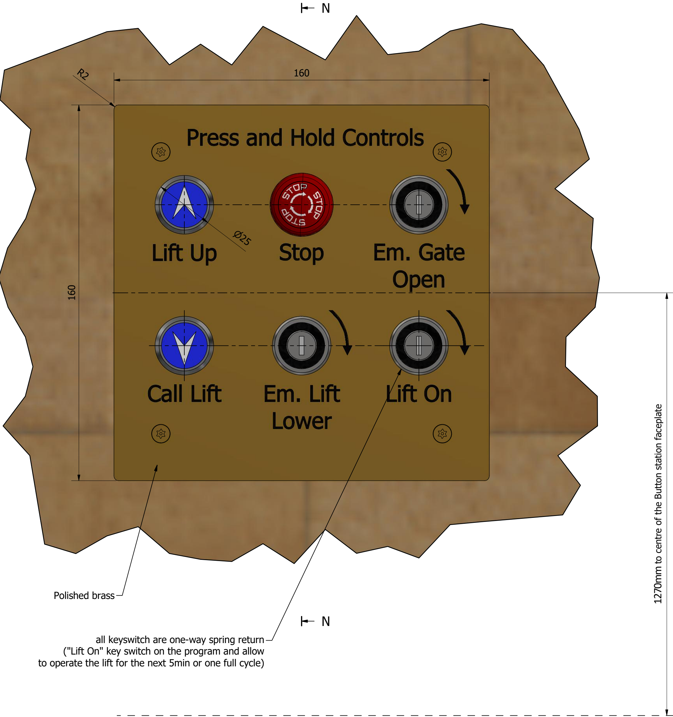
Removable Hand Held Post ( 1 : 2 )
