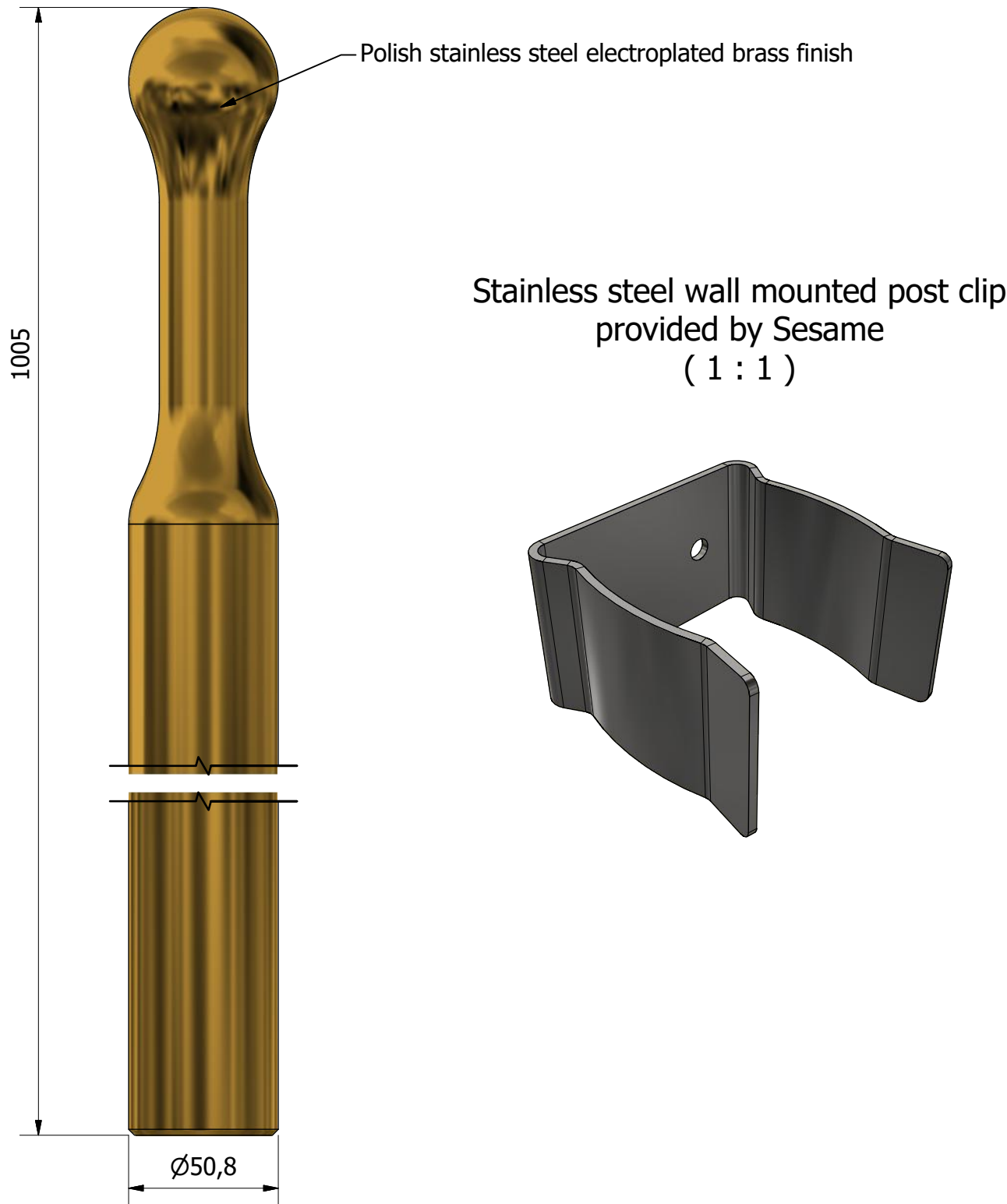
Removable Hand Held Post ( 1 : 2 )
