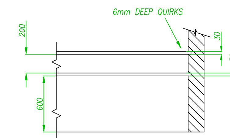
DIMENSIONS AT SIDE OF STEPS
