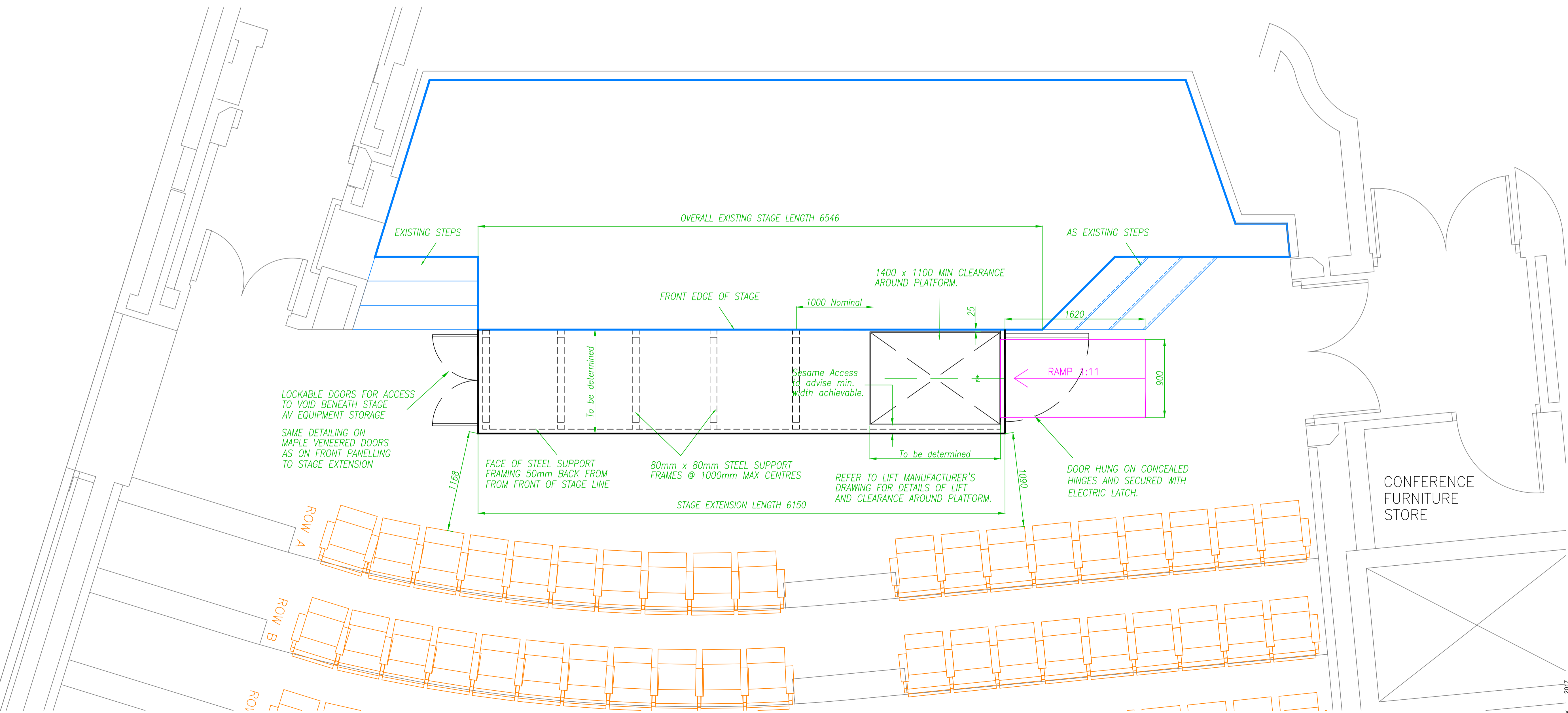
PROPOSED PLAN OF STAGE EXTENSION INCORPORATING PLATFORM LIFT
