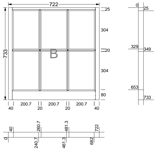
KP5 Bottom sliding sash
