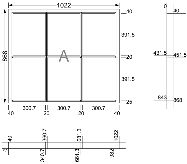
KP3 Top sliding sash
