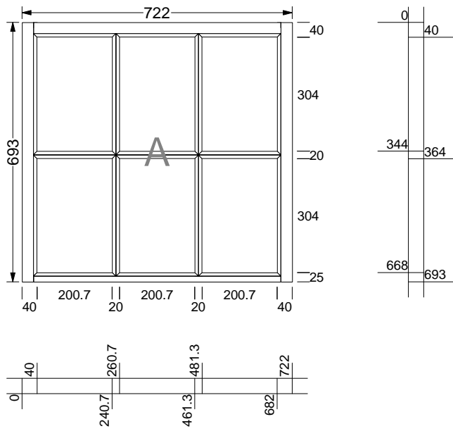
KP5 Top sliding sash
