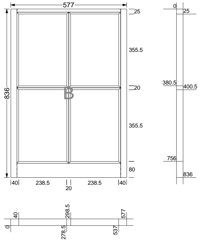
KP4 Bottom sliding sash
