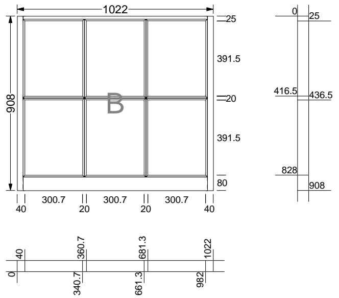
KP3 Bottom sliding sash
