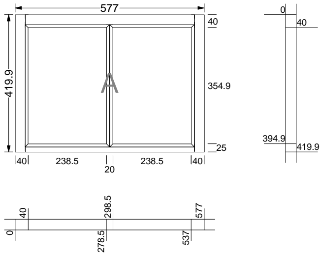
KP4 Top sliding sash
