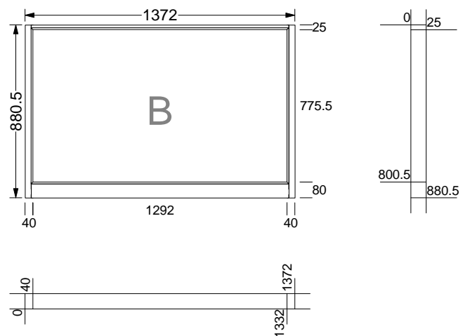
KP7 Bottom sliding sash
