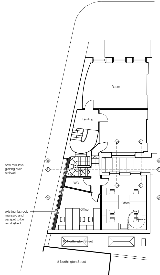
FIRST FLOOR 1:50
