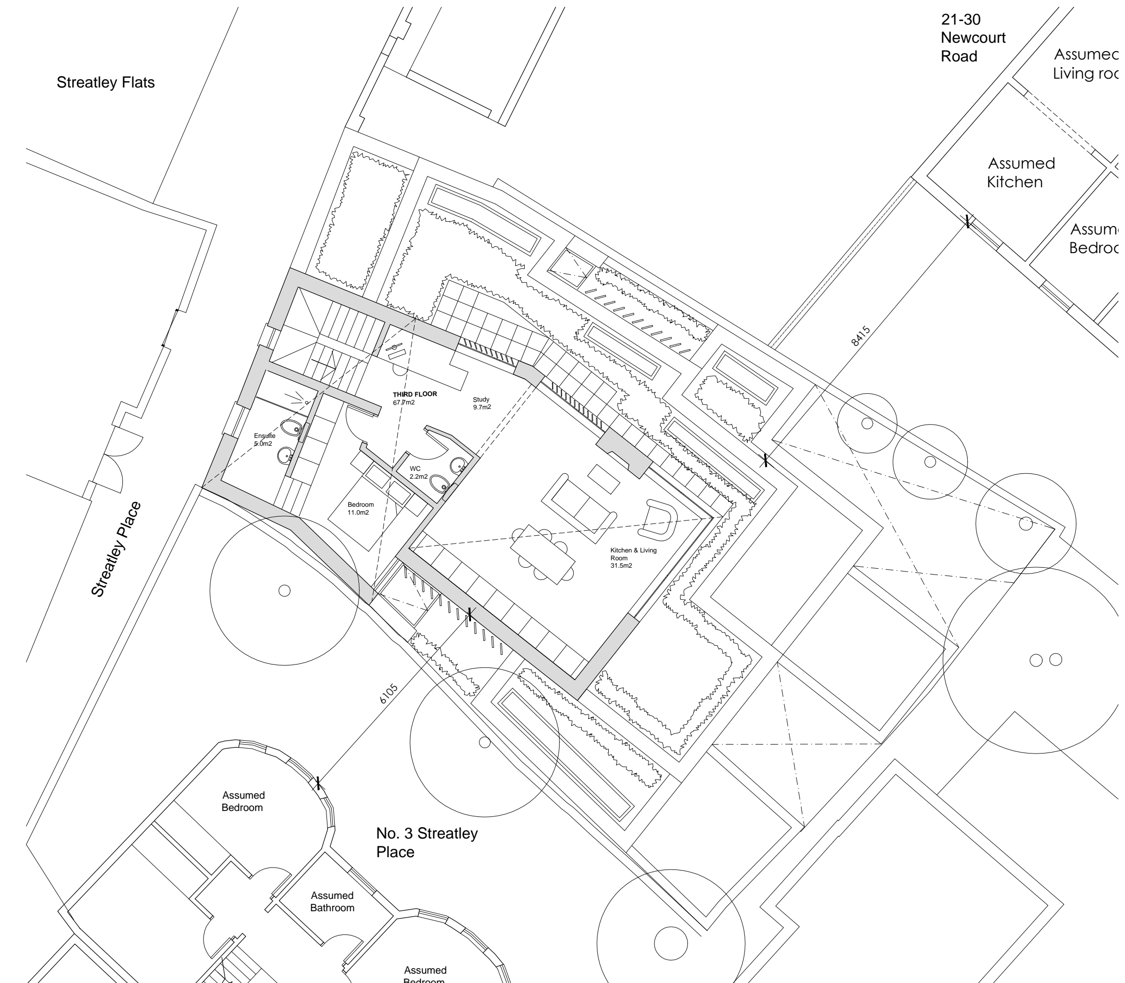
Proposed Second Floor Plan 1:100 @ A3 & 1:50 @ A1
