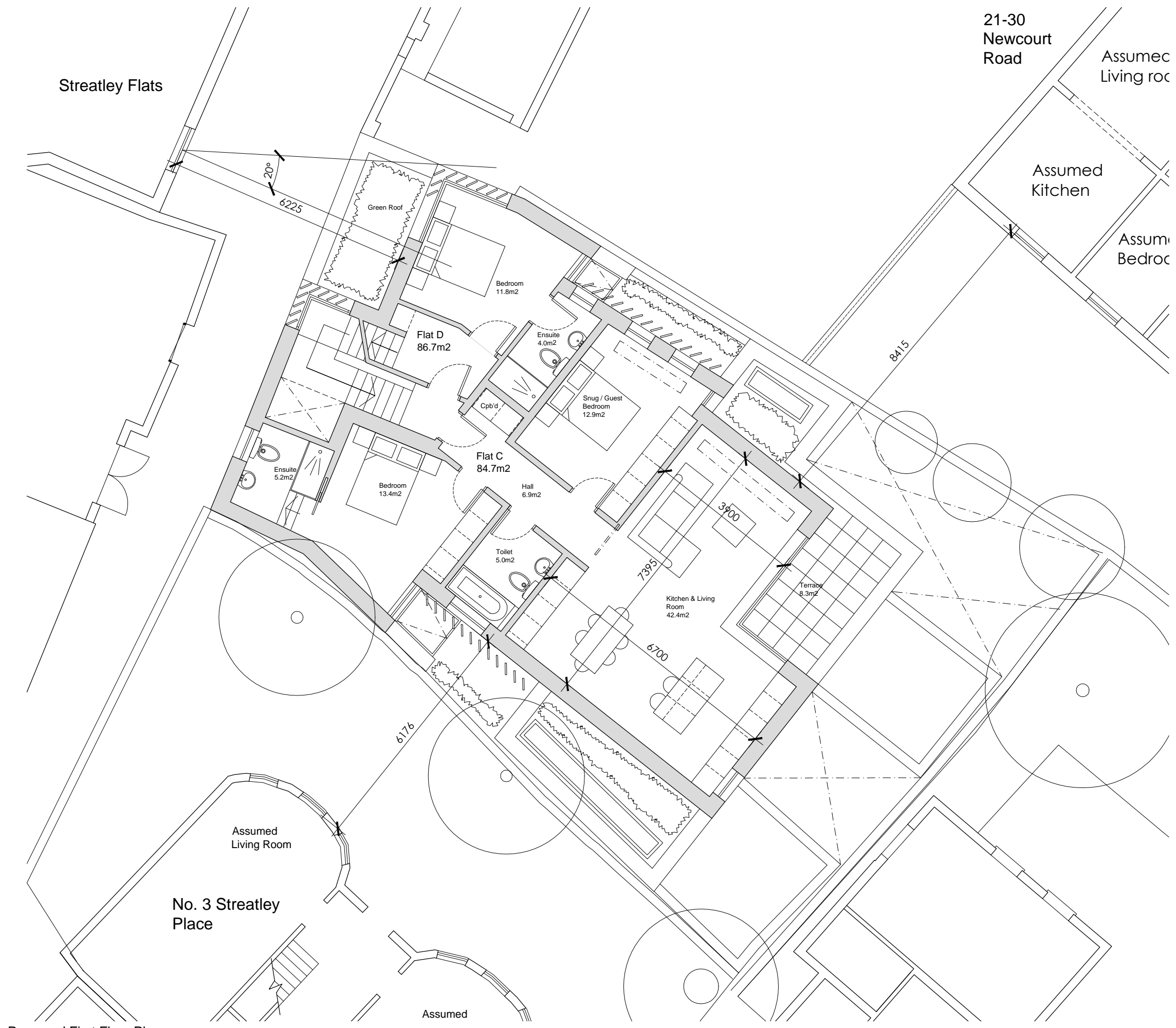
Proposed First Floor Plan 1:100 @ A3 & 1:50 @ A1
