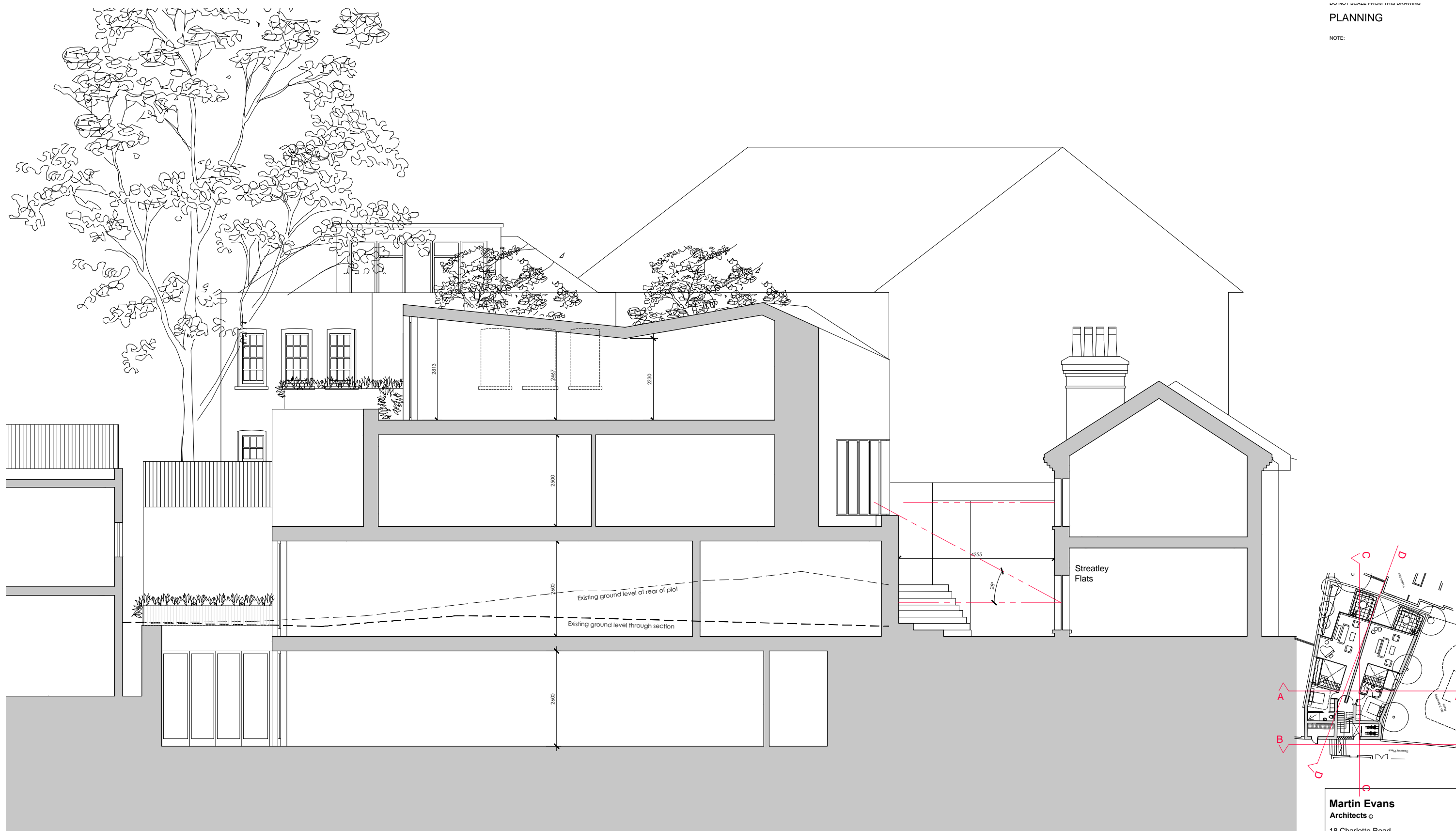
Proposed elevation D - Side Elevation 1:100 @ A3 & 1:50 @ A1
