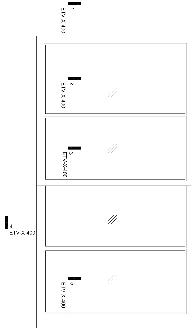
TYPICAL SASHES (FRONT ELEVAT.) 1 1:10 @ A3 ETV-X-401
