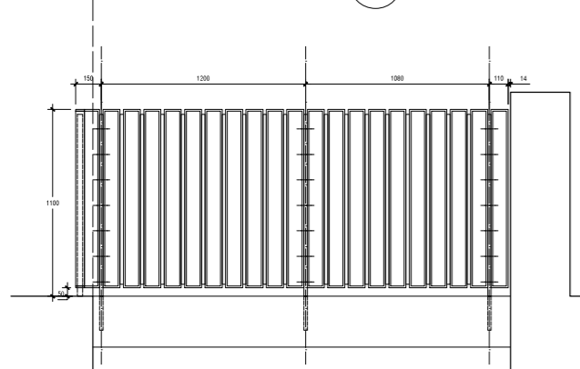
DETAIL PLAN AND ELEVATION 10 SCALE: 1:5
