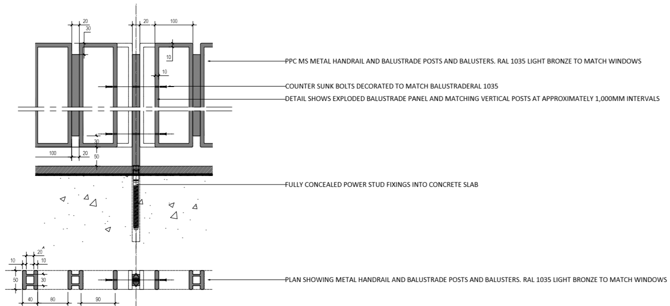
DETAIL PLAN AND ELEVATION 10 SCALE: 1:5
